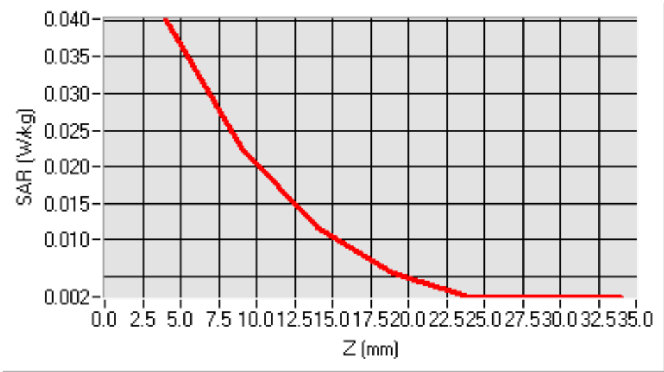
SAR, Z Axis Scan (X = -10, Y = -36)
