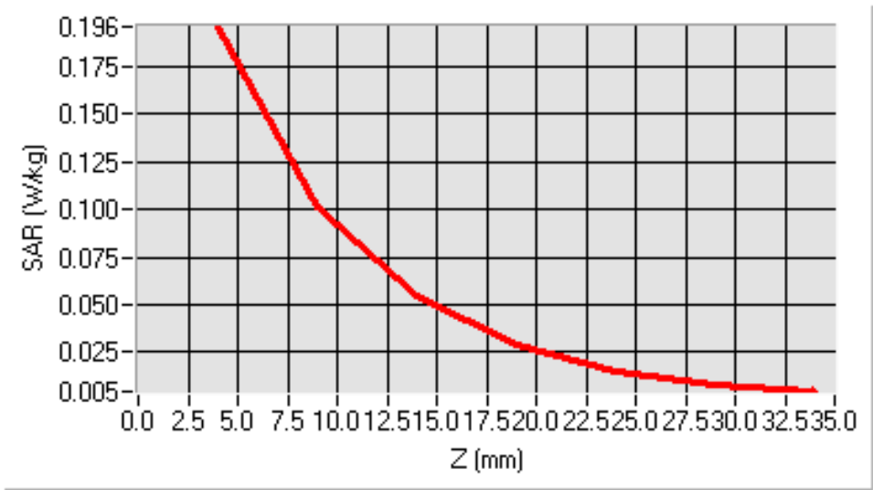
SAR, Z Axis Scan (X = -9, Y = -35)
