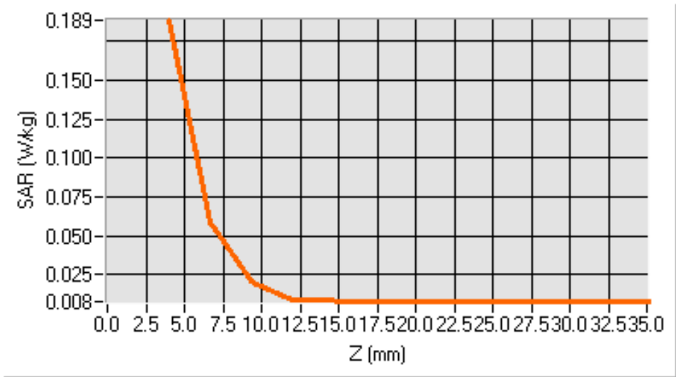
SAR, Z Axis Scan (X = -23, Y = -39)
