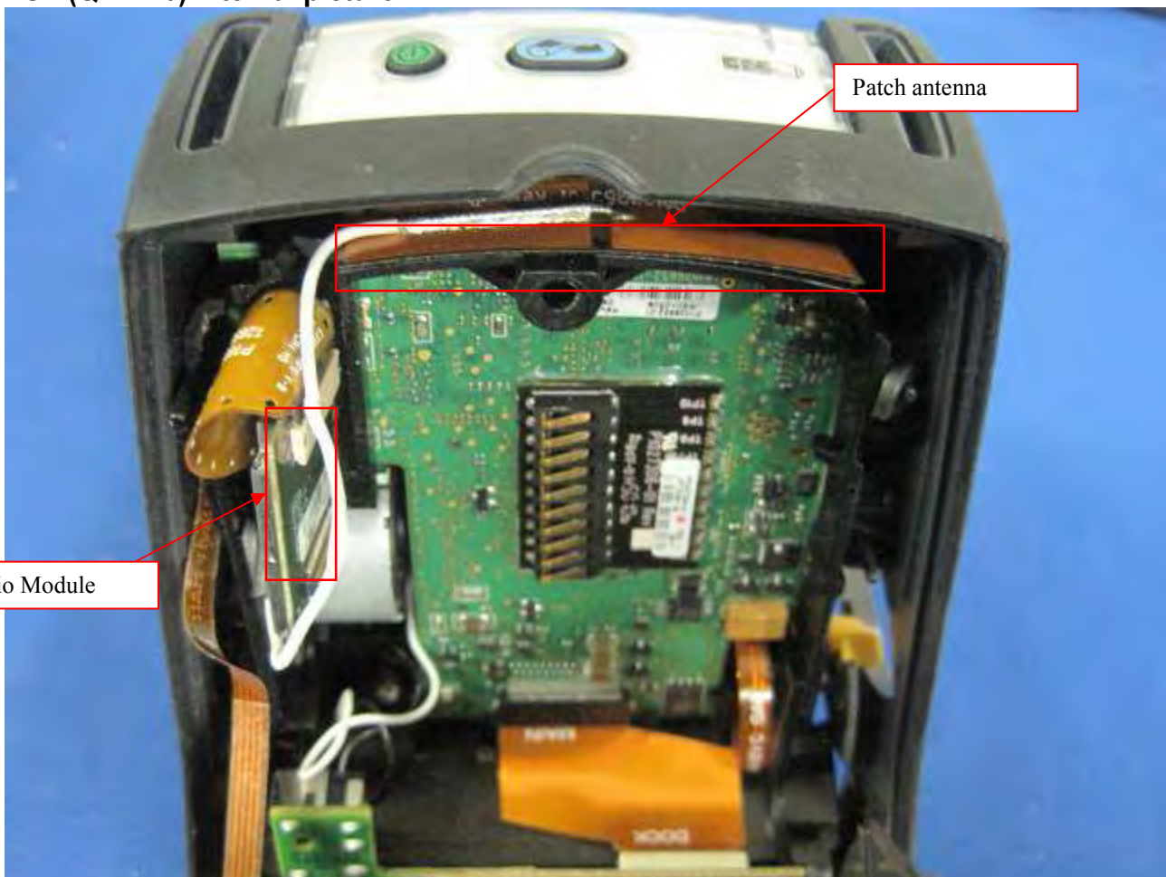
QLn220 Internal View
