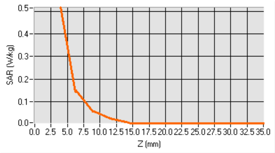
SAR, Z Axis Scan (X = 26, Y = -31)
