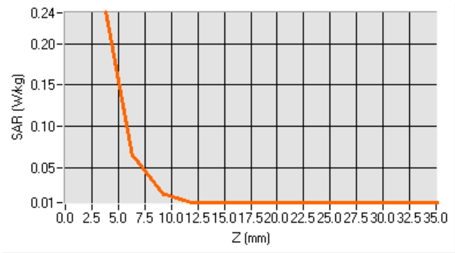
SAR, Z Axis Scan (X = 30, Y = -31)
