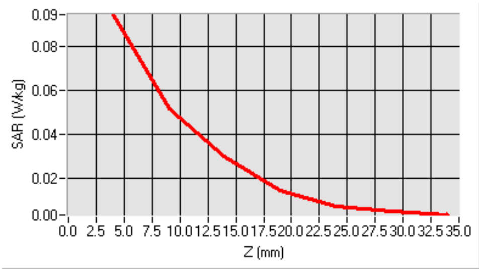
SAR, Z Axis Scan (X = 13, Y = -59)
