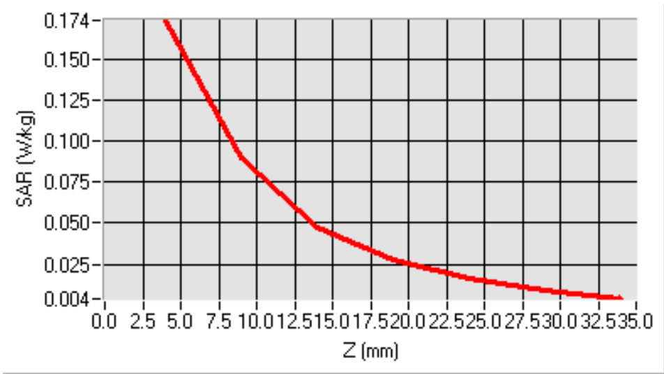
SAR, Z Axis Scan (X = -9, Y = -34)
