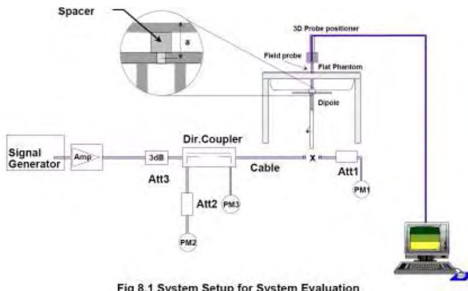
Fig 8.1 System Setup for System Evaluation
