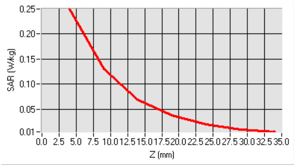
SAR, Z Axis Scan (X = -9, Y = -36)
