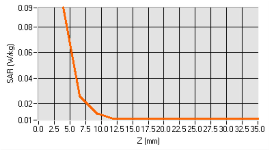
SAR, Z Axis Scan (X = 16, Y = -62)
