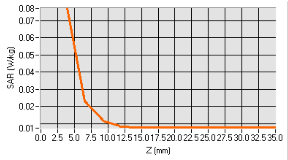
SAR, Z Axis Scan (X = 16, Y = -63)
