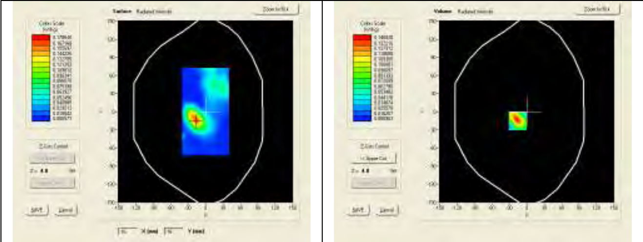
SAR, Z Axis Scan (X = -16, Y = -15)
