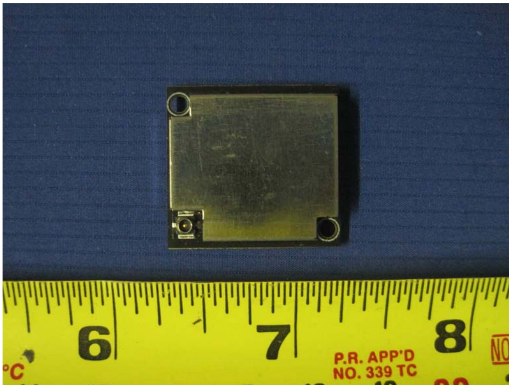
Radio Board Top View
