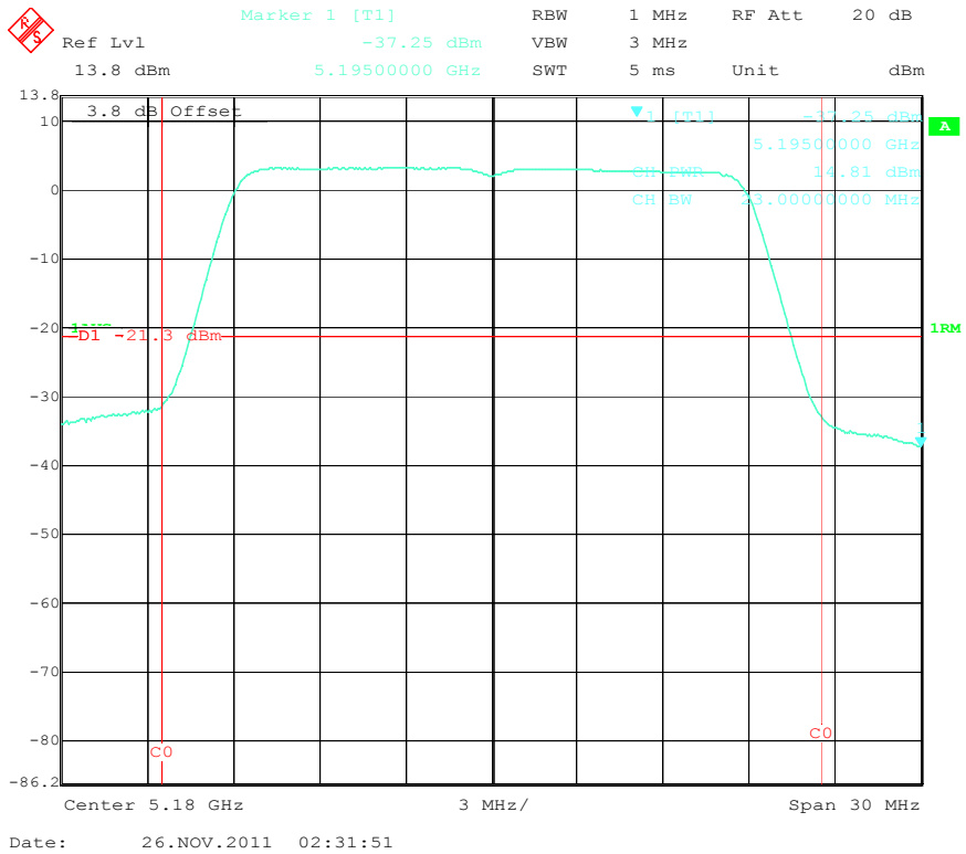
Output Power Low Channel (N mode – 20MHz, 5.2GHz)
