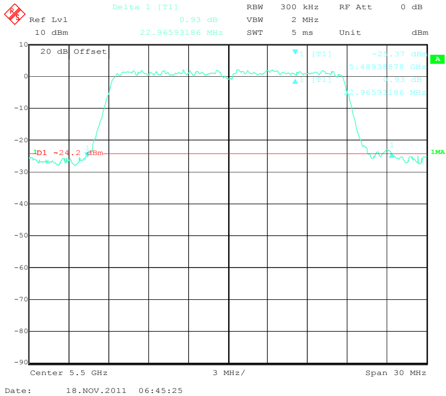
26 dB Bandwidth Low Channel (802.11n-20MHz-5.6G-5500MHz)
