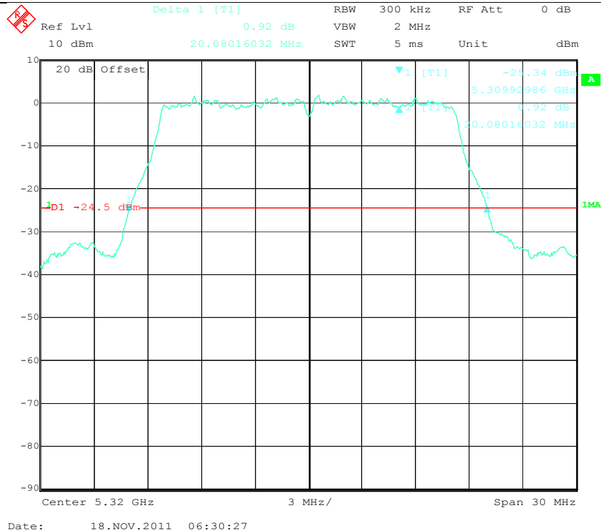
26 dB Bandwidth - High Channel (802.11a-5.2G-5320MHz)
