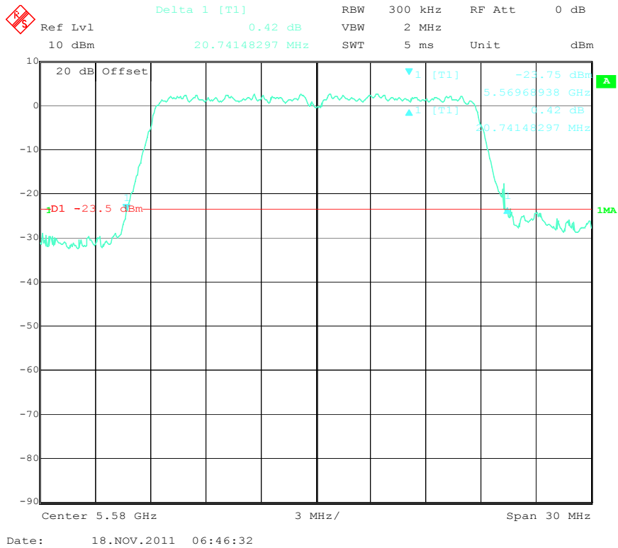
26 dB Bandwidth Mid Channel (802.11n-20MHz-5.6G-5580MHz)
