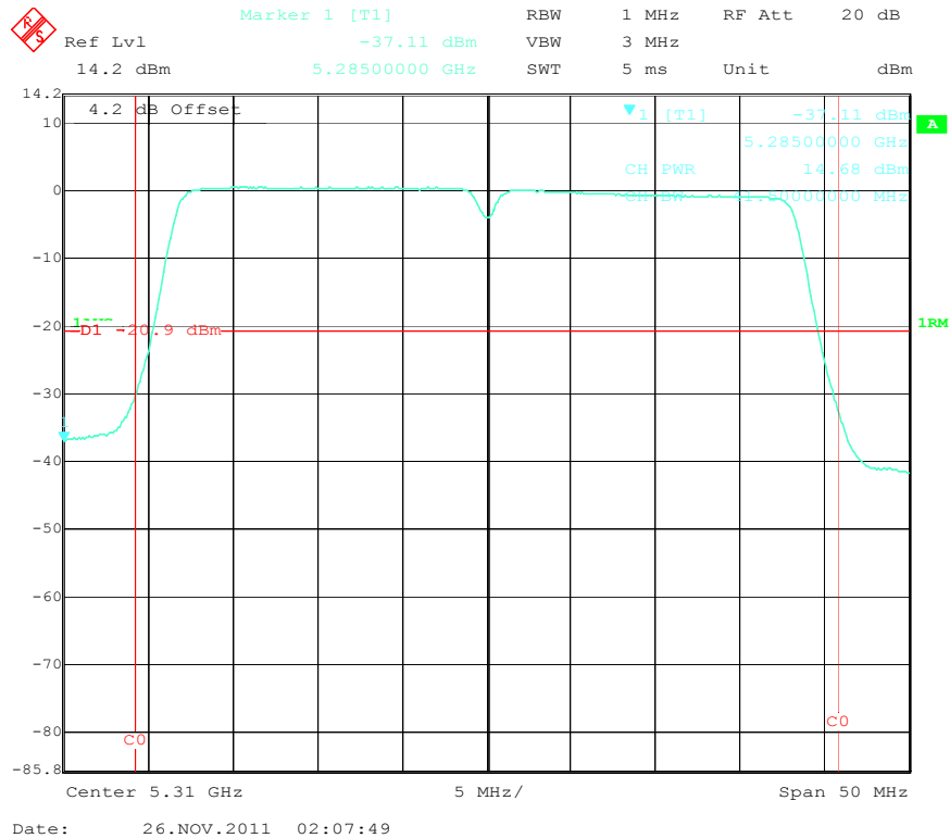
Output Power High Channel (N mode-40MHz, 5.3GHz)
