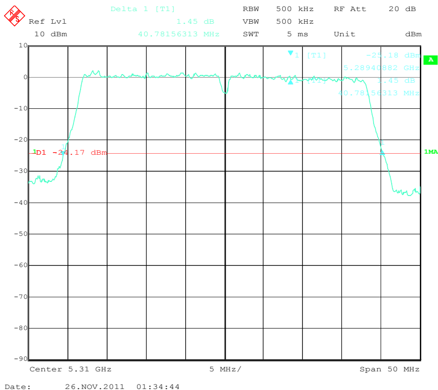
26 dB Band Width High Channel (802.11n-40MHz-5.2G-5310MHz)
