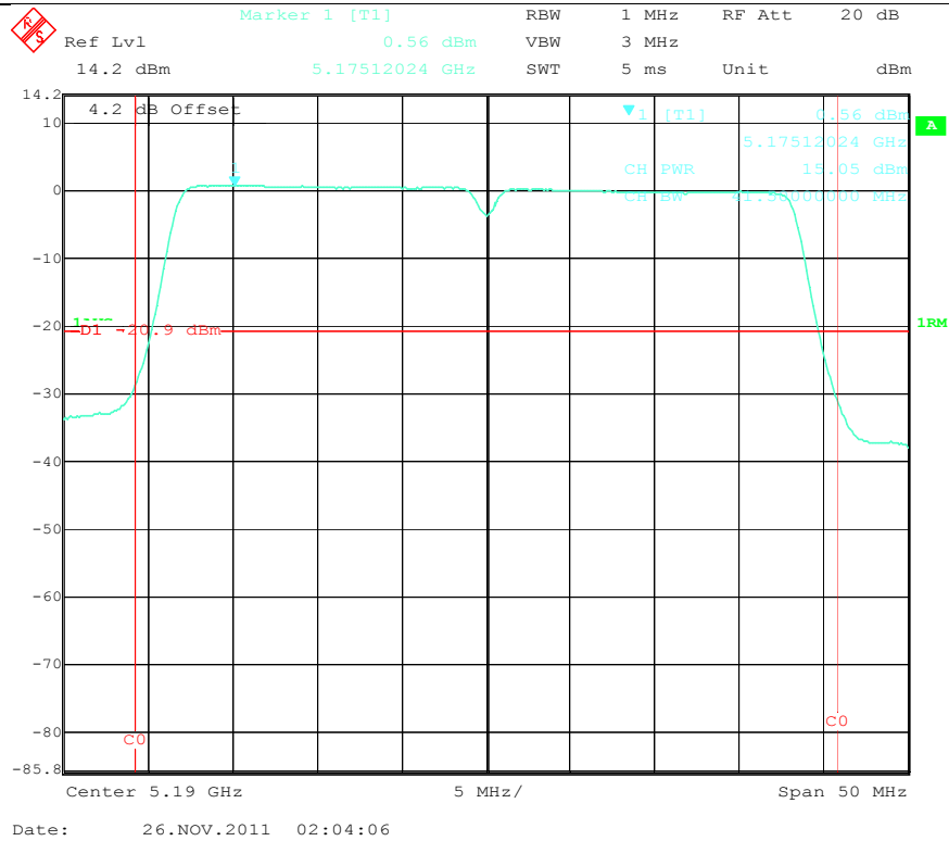
Output Power Low Channel (N mode – 40MHz, 5.2GHz)
