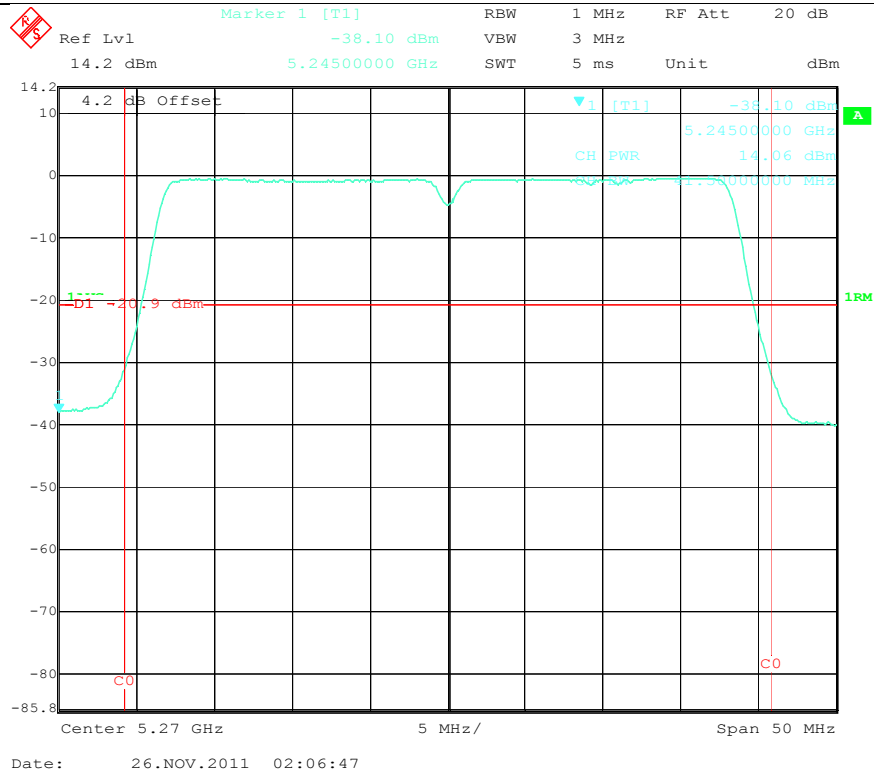
Output Power Low Channel (N mode - 40MHz, 5.3GHz)
