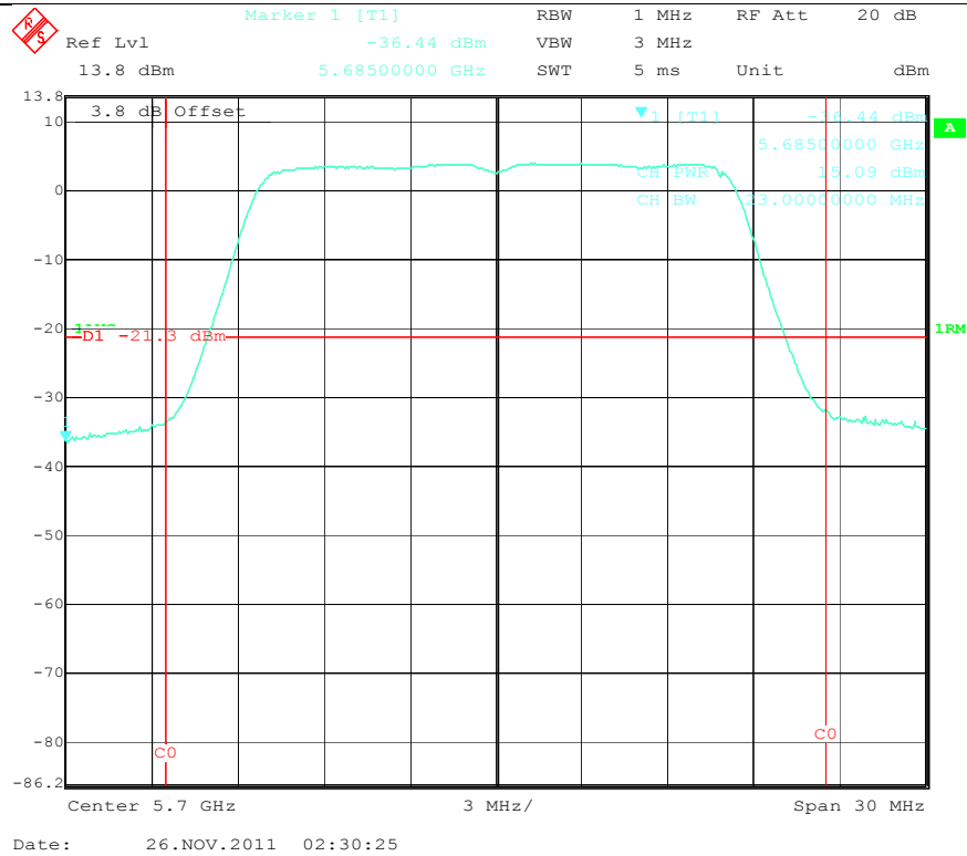
Output Power High Channel (A mode-20MHz, 5.6GHz)
