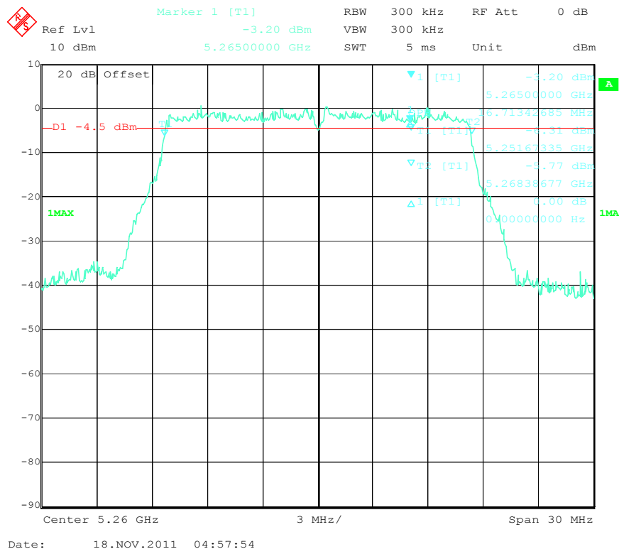
99% Band Width Low Channel (802.11a-5.2G-5260MHz)
