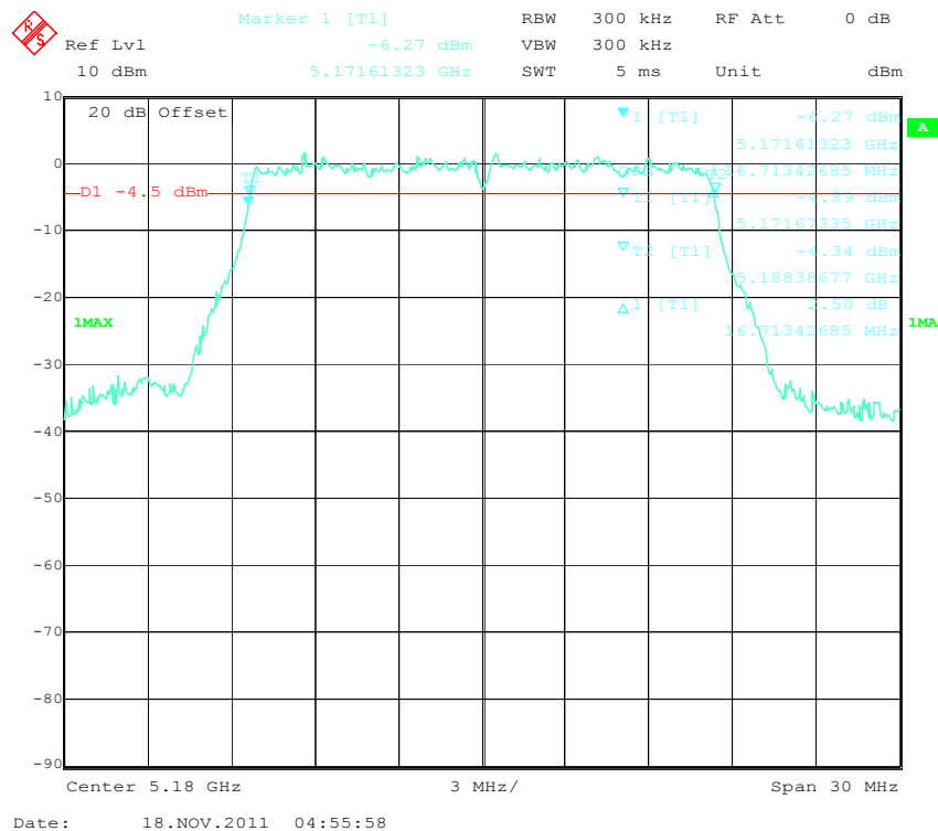
99% Band Width Low Channel (802.11a-5.1G-5180MHz)
