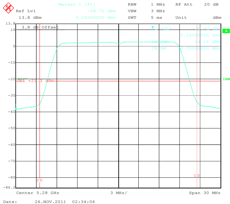
Output Power Mid Channel (N mode-20MHz, 5.3GHz)
