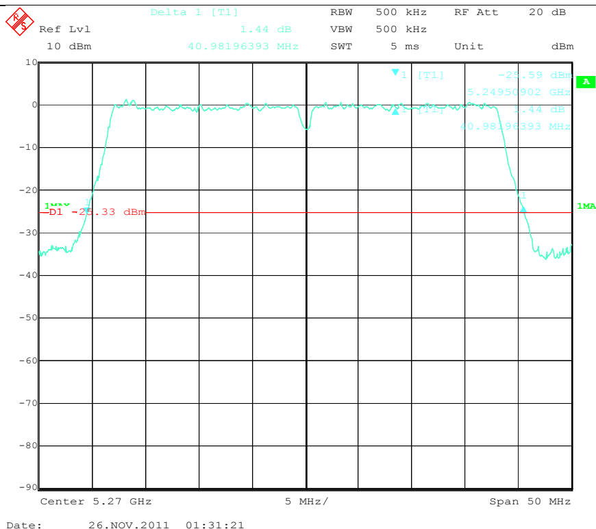
26dB Band Width Low Channel (802.11n-40MHz-5.2G-5270MHz)
