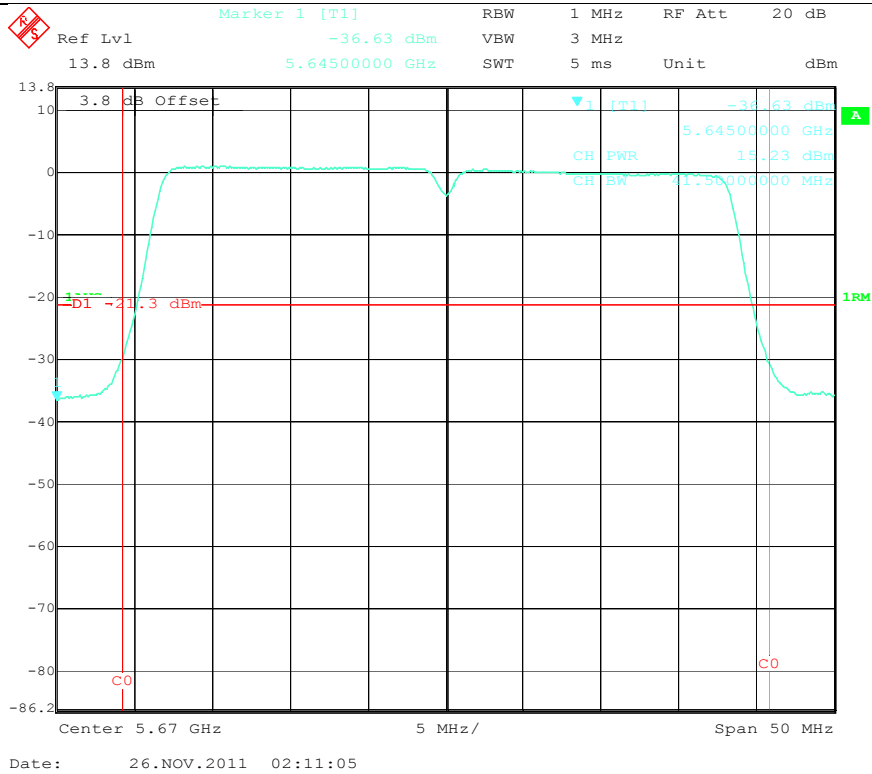
Output Power High Channel (N mode-40MHz, 5.6GHz)
