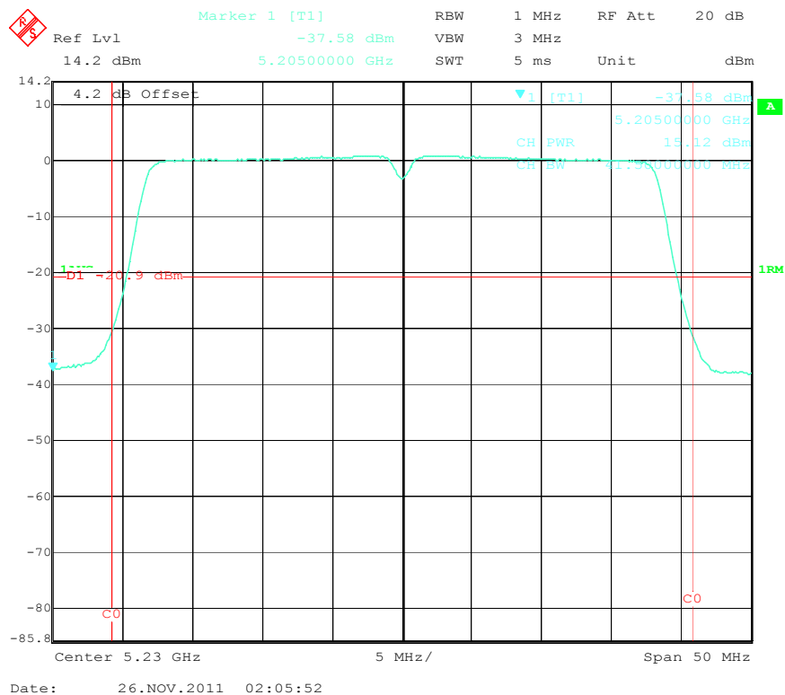
Output Power High Channel (N mode-40MHz, 5.2GHz)
