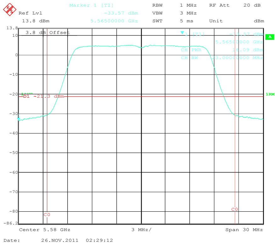
Output Power Mid Channel (A mode-20MHz, 5.6GHz)
