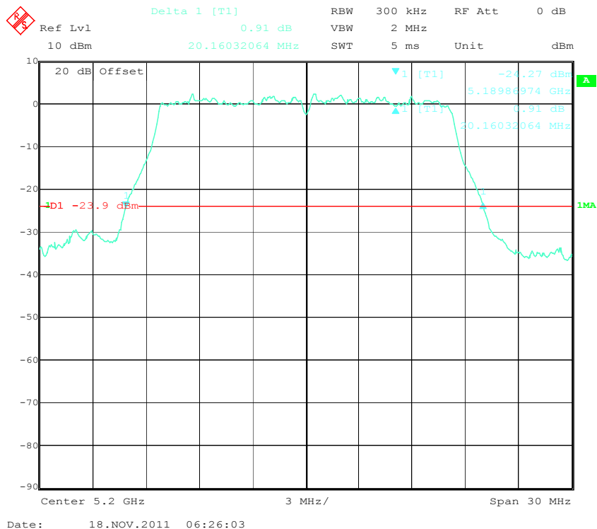
26 dB Bandwidth - Mid Channel (802.11a-5.1G-5200MHz)
