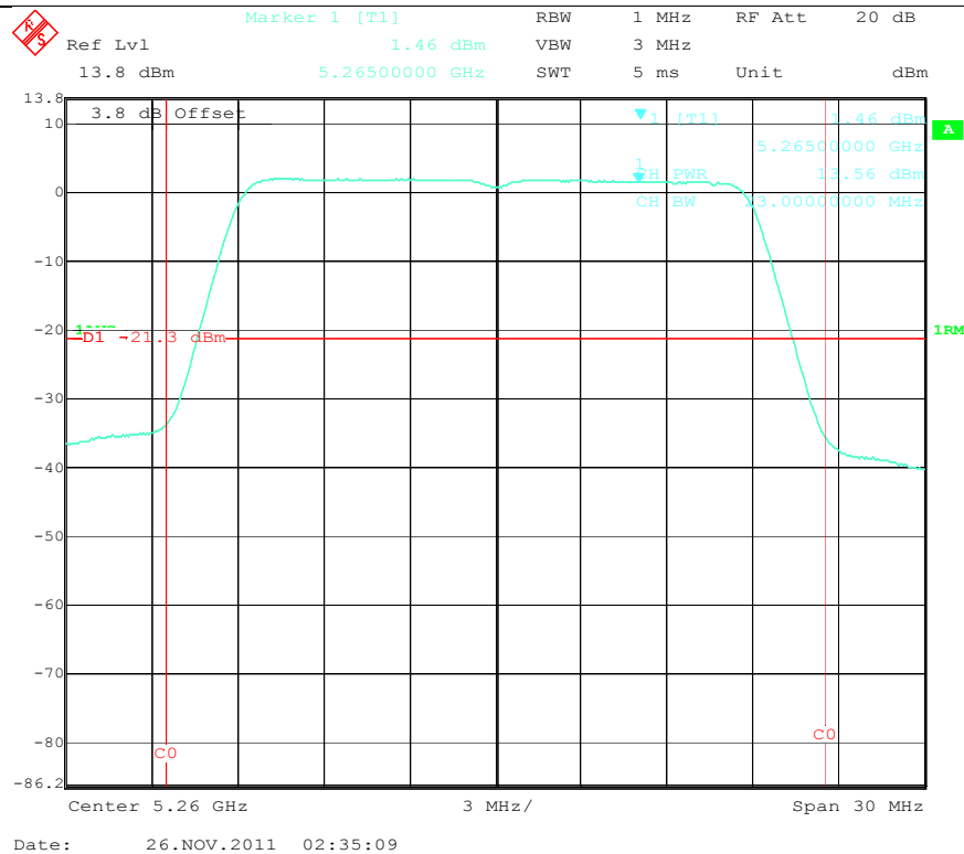
Output Power Low Channel (N mode – 20MHz, 5.3GHz)
