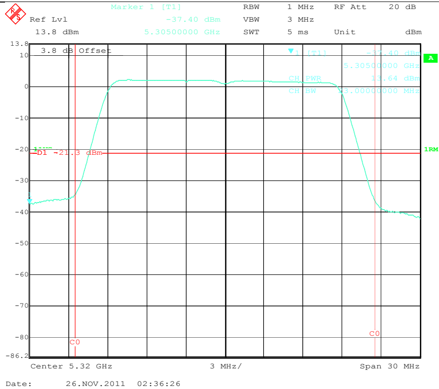
Output Power High Channel (N mode-20MHz, 5.3GHz)
