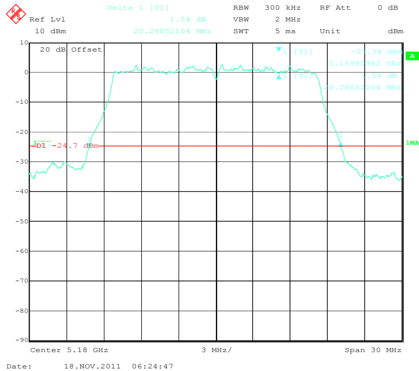
26 dB Bandwidth - Low Channel (802.11a-5.1G-5180MHz)
