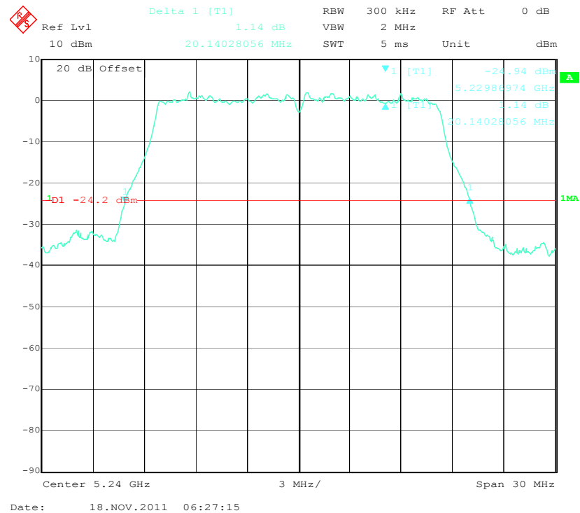
26 dB Bandwidth - High Channel (802.11a-5.1G-5240MHz)
