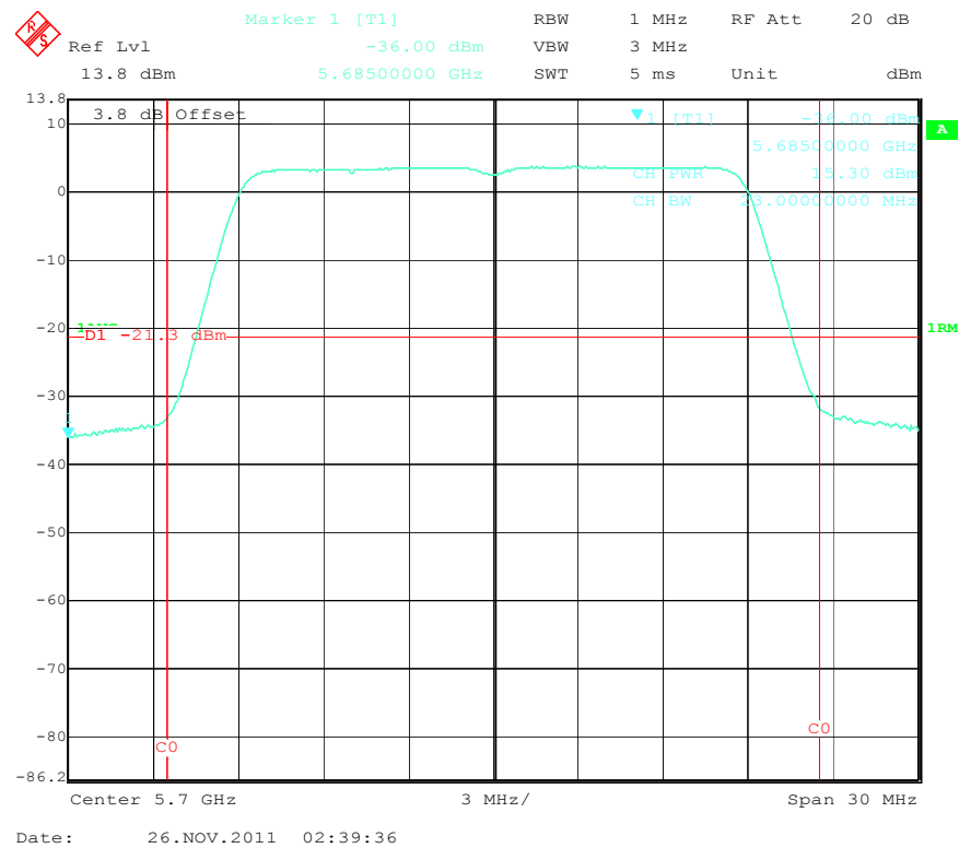
Output Power High Channel (N mode-20MHz, 5.6GHz)
