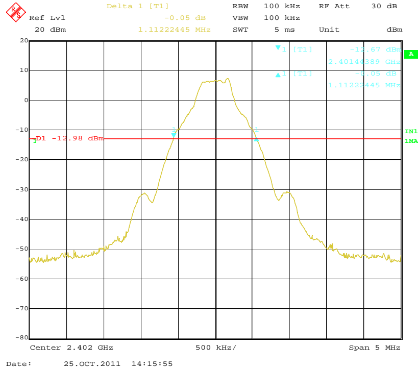
20dB Bandwidth - Low Channel (Basic Rate)
