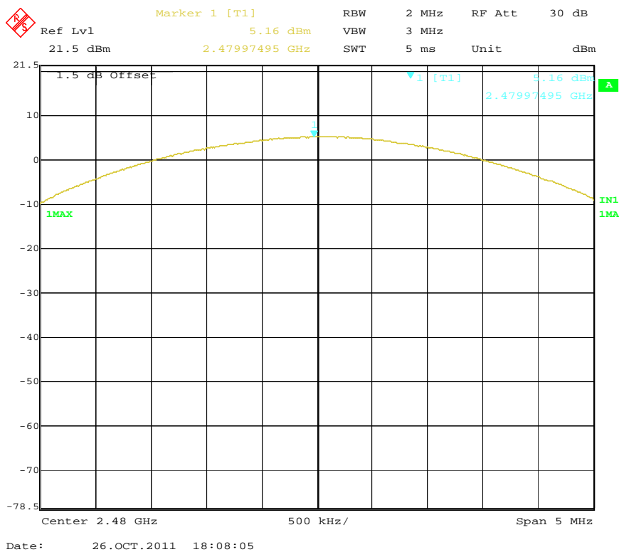
Output Power High Channel (Bluetooth)
