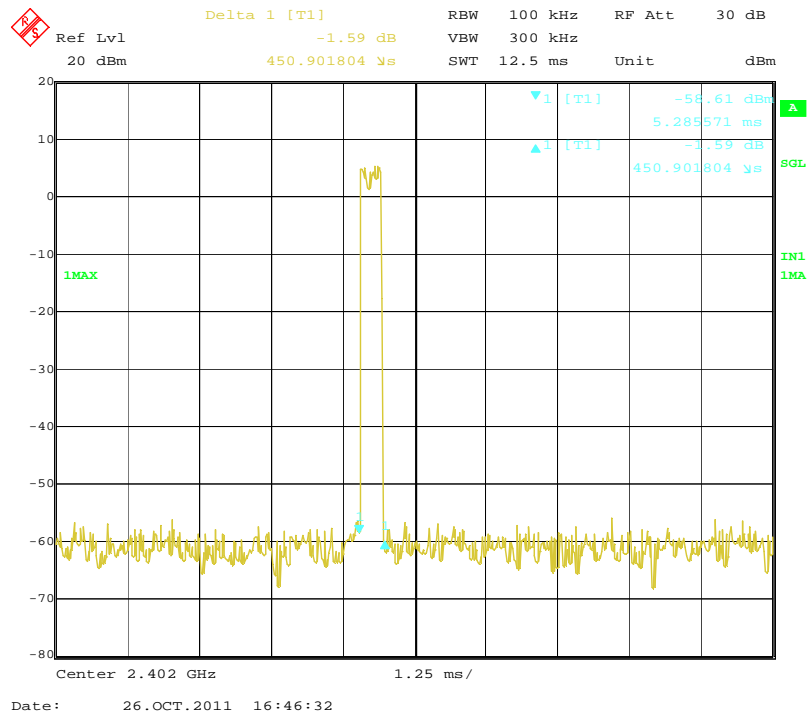
Low Channel (Sweep in 12.5msec)
