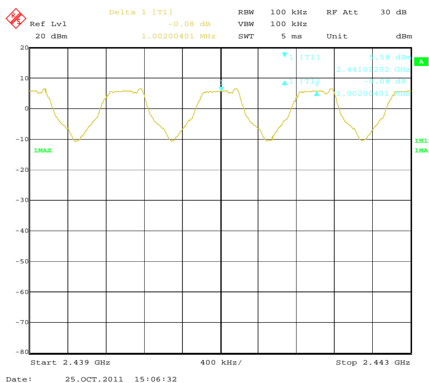
Channel Separation - Middle Channel (Basic Data Rate, 1Mbps)
