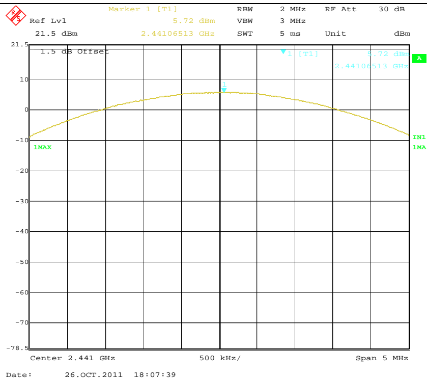
Output Power Mid Channel (Bluetooth)
