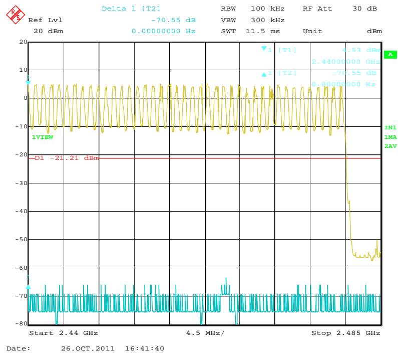
40-Channel (cont. of Graph 1)
