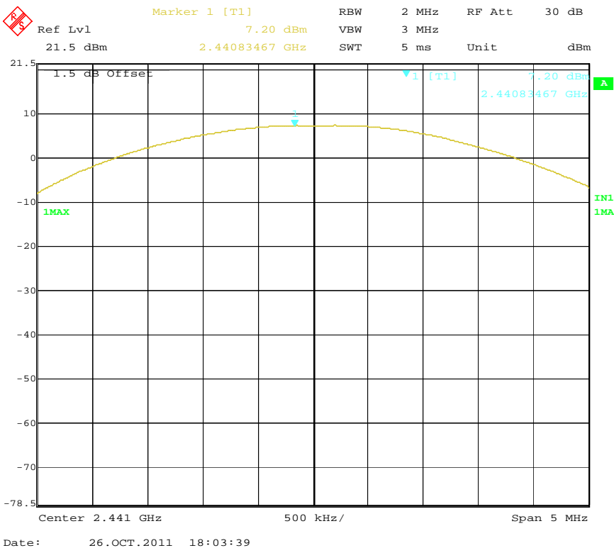
Output Power Middle Channel (Bluetooth)
