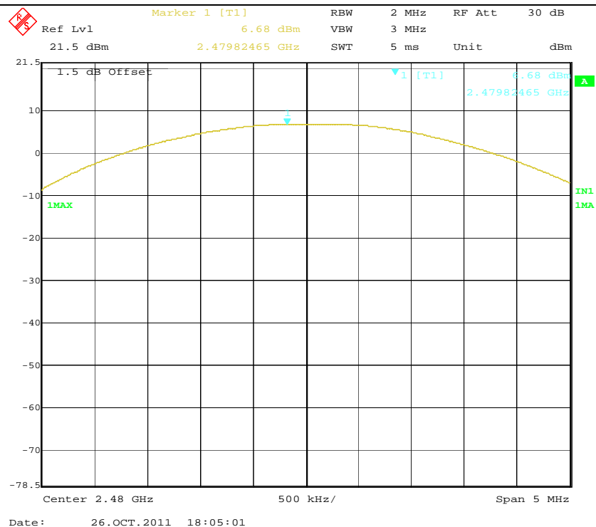
Output Power High Channel (Bluetooth)
