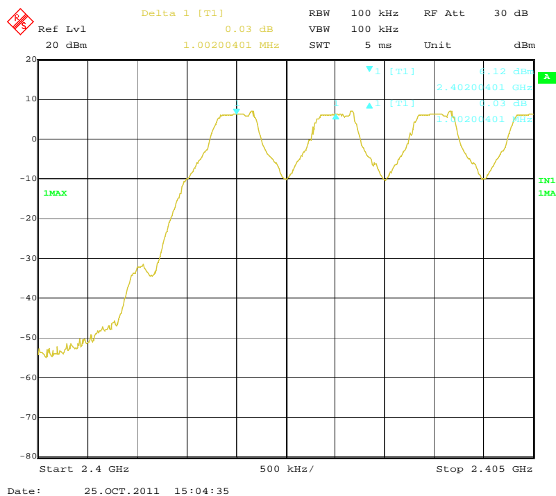
Channel Separation - Low Channel (Basic Data Rate, 1Mbps)
