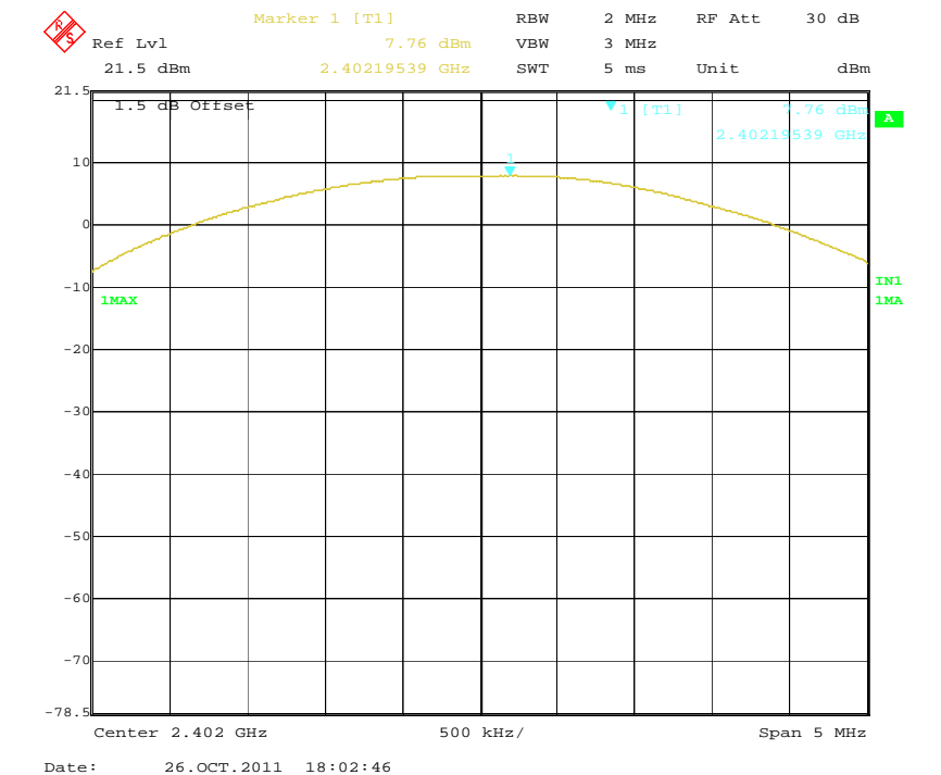
Output Power Low Channel (Bluetooth)
