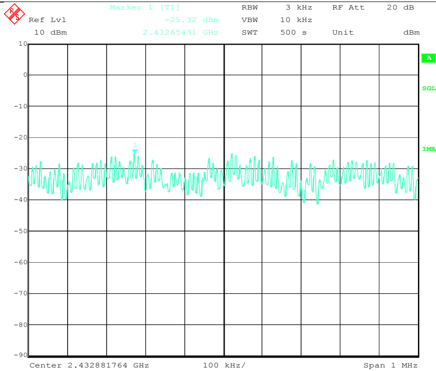
PSD Mid Channel ( 802.11g)
