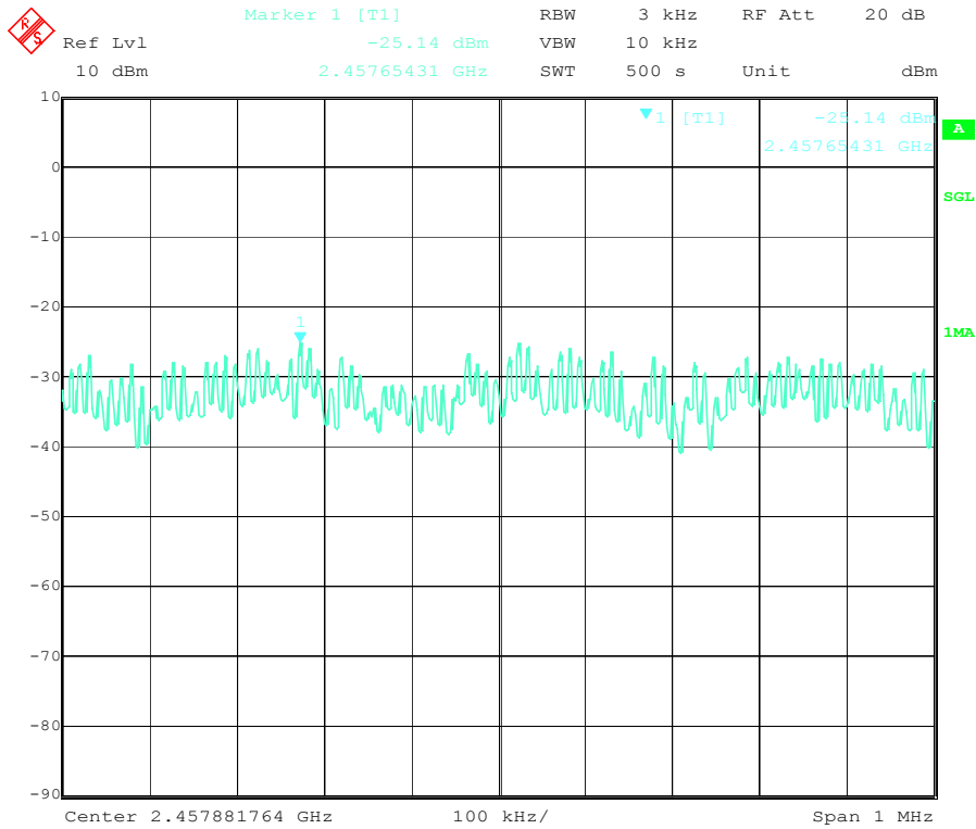
PSD High Channel ( 802.11g)
