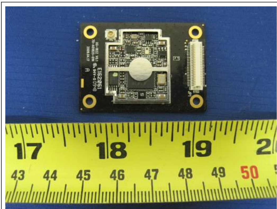
EUT – without RF shield
