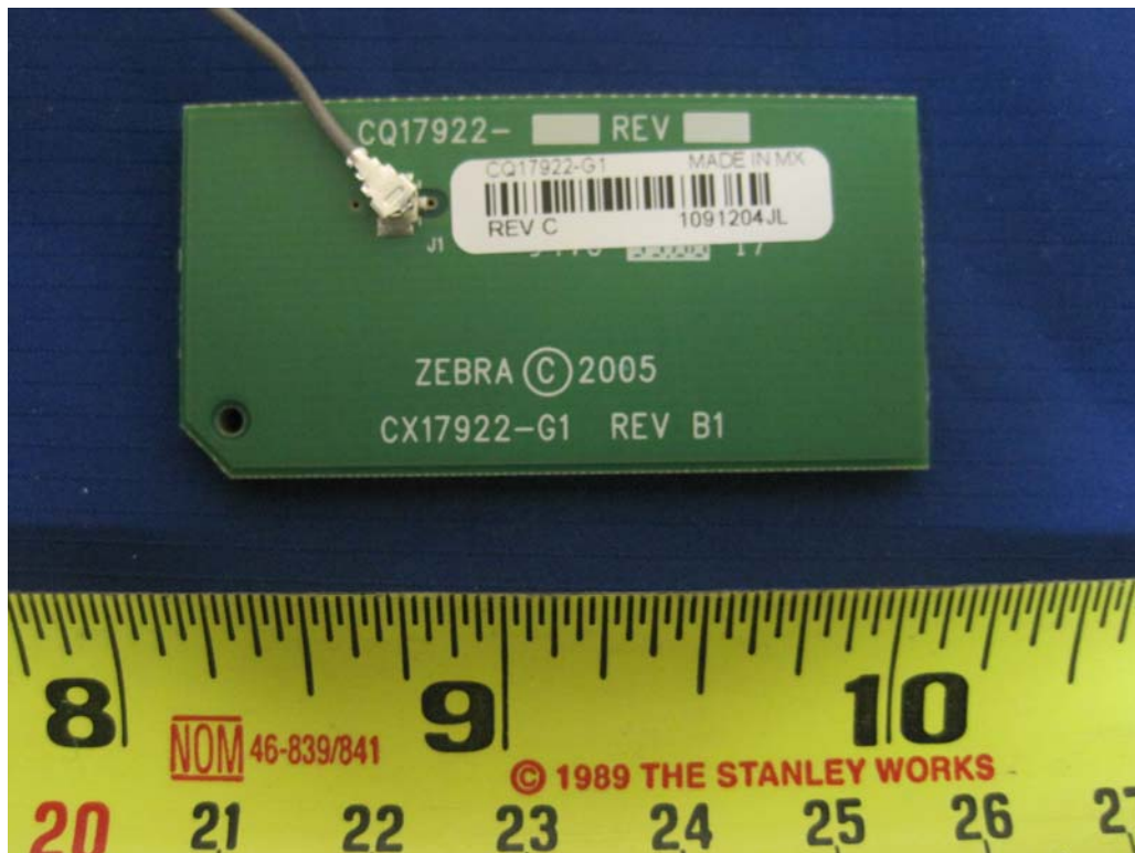
EUT: Antenna bottom view
