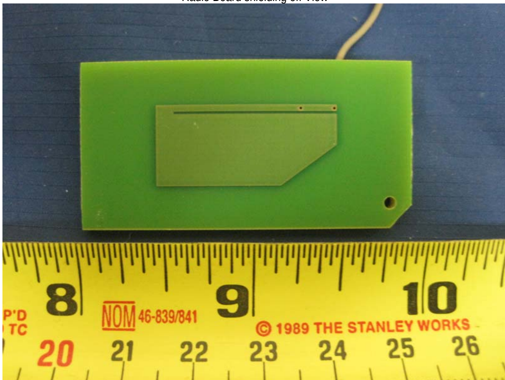
EUT: Antenna top view
