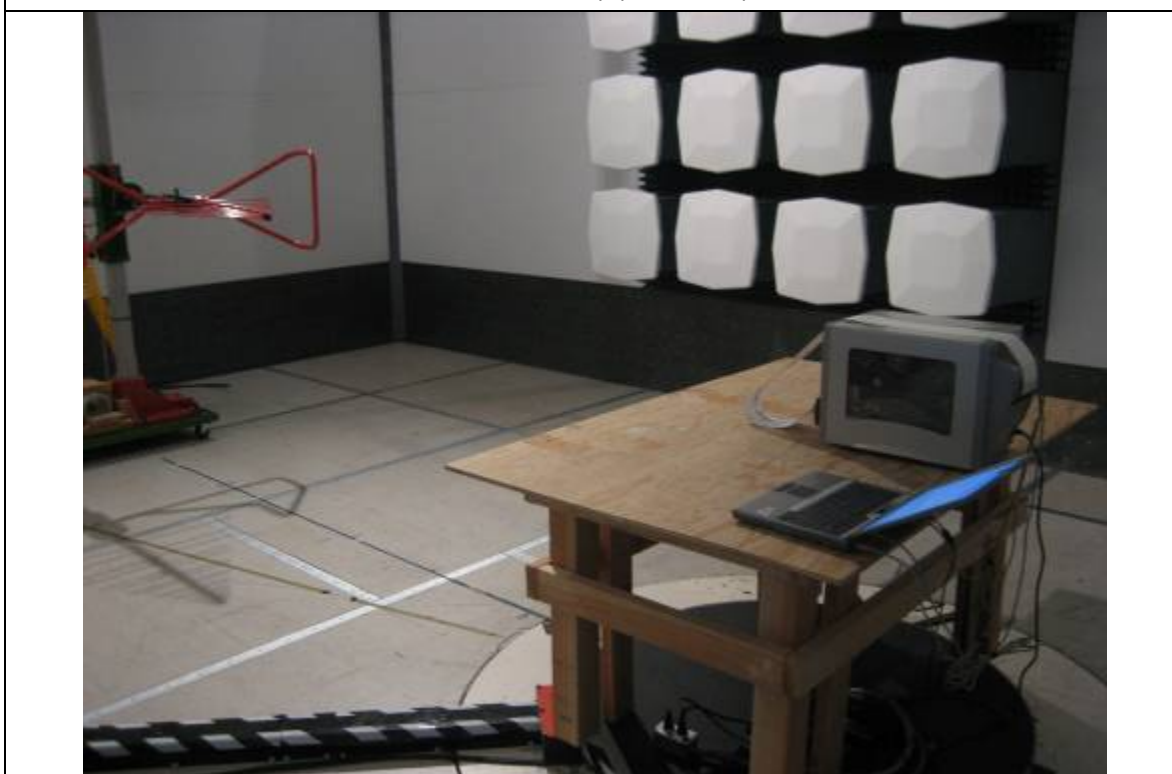
Radiated Emission Test Setup (above 1GHz) – Rear View
