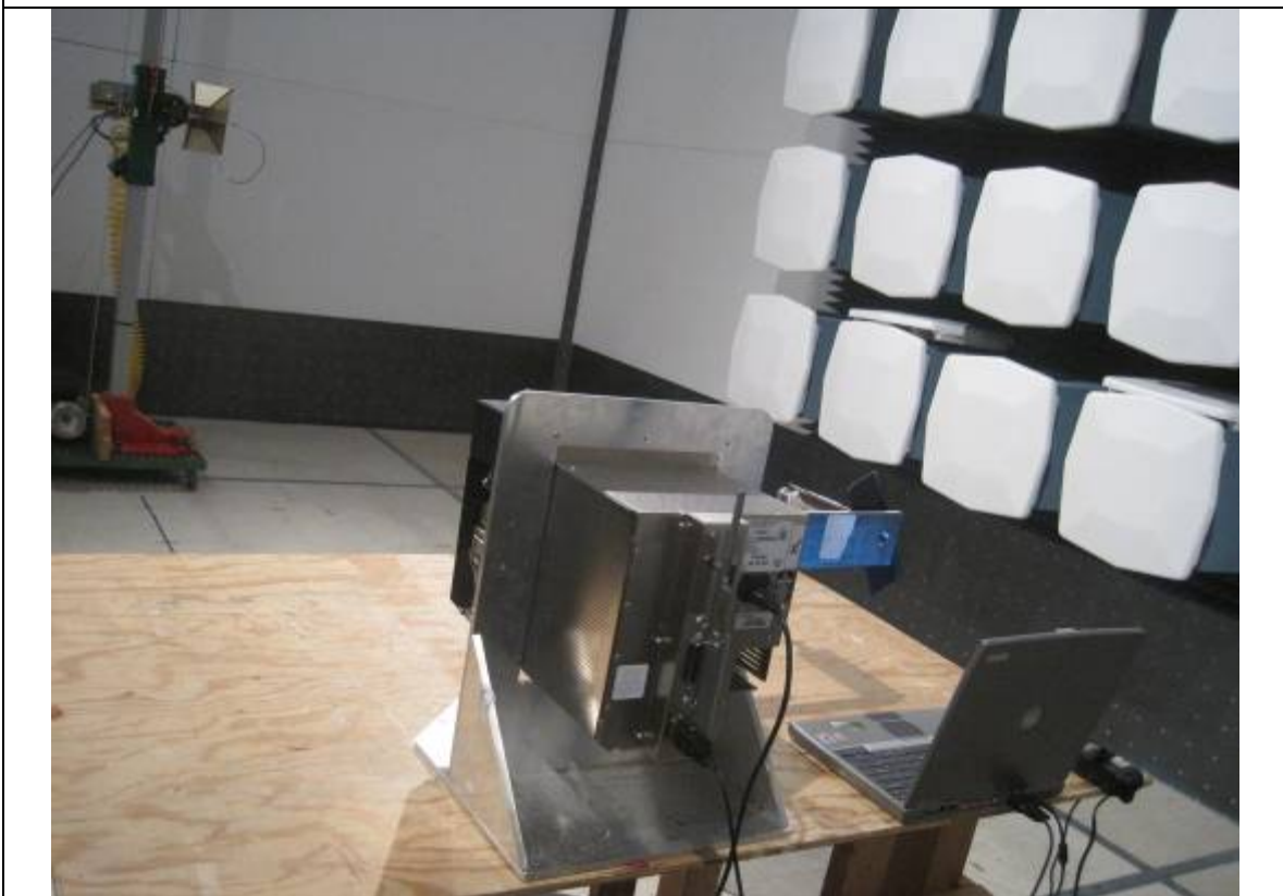
Radiated Emission Test Setup (above 1GHz) – Rear View
