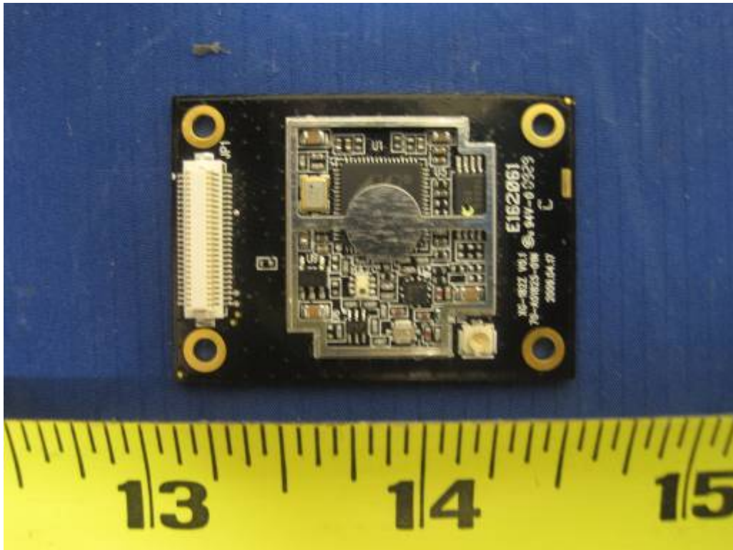
EUT – WLAN Module Component PCBA View
