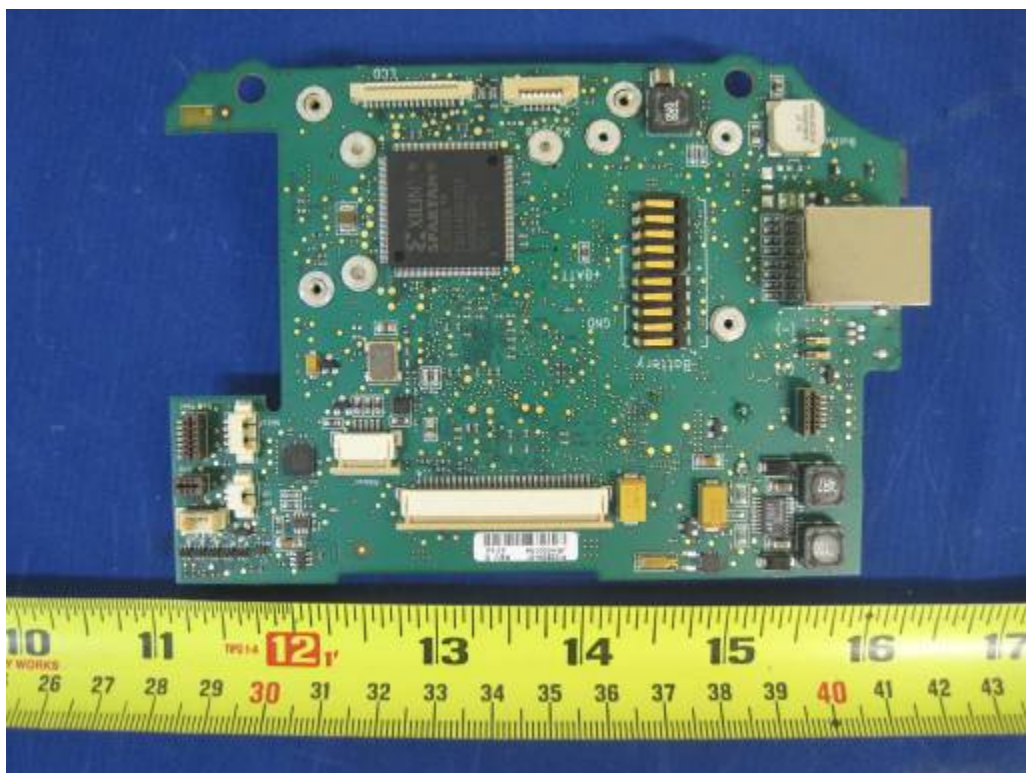
EUT – Main PCBA Solder View
