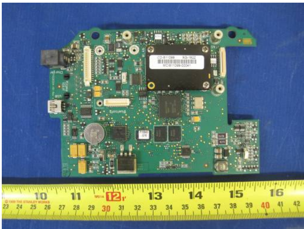
EUT – Main PCBA Component View
