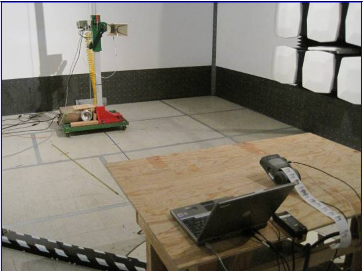
Host: QL 320plus Radiated Emission Test Setup – Rear View
