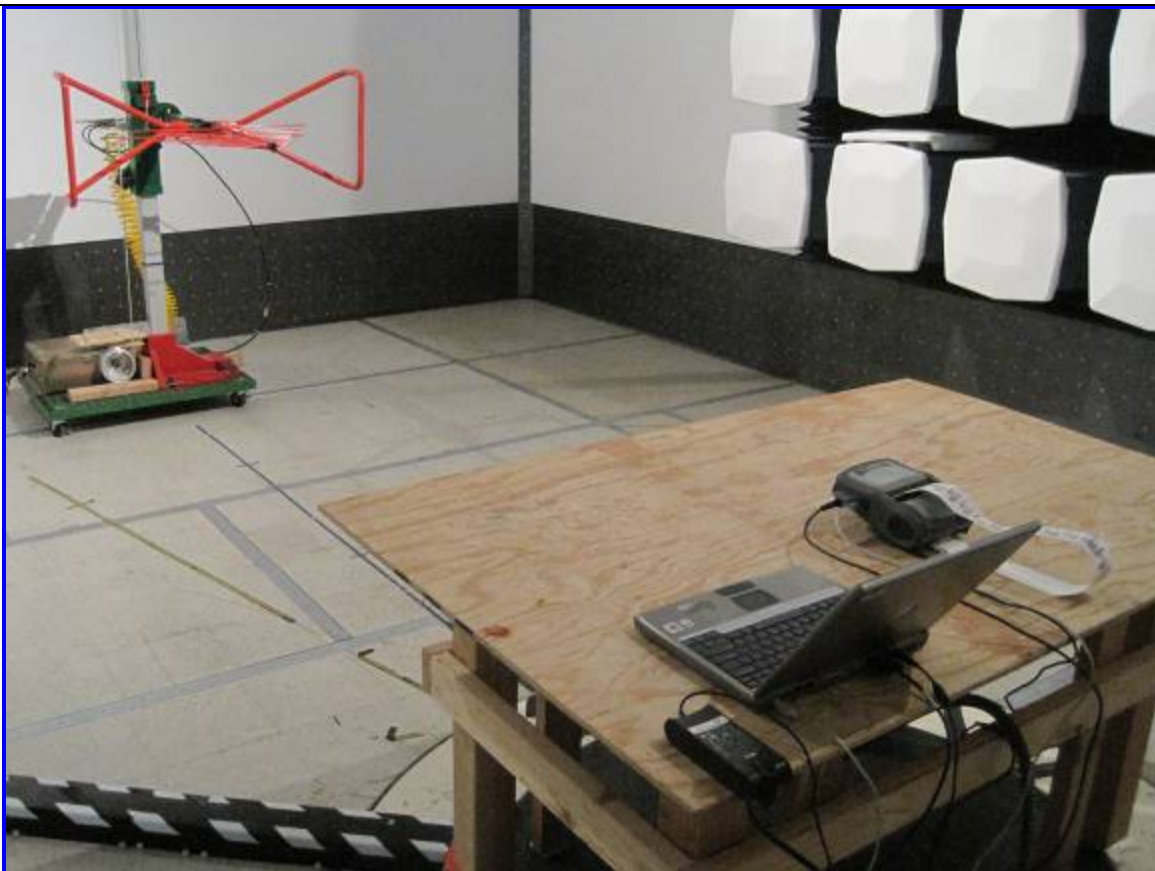
Host: QL 420plus Radiated Emission Test Setup – Rear View
