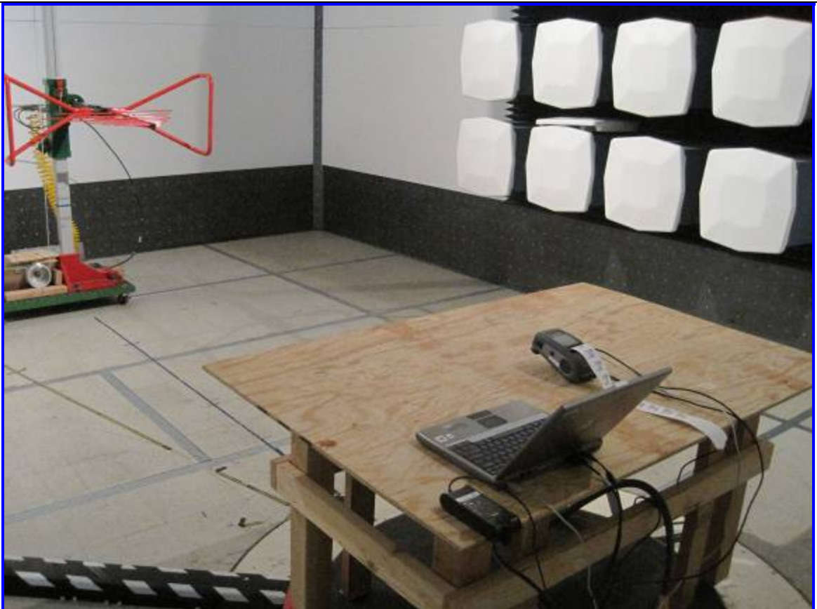
Host: QL 220plus Radiated Emission Test Setup – Rear View
