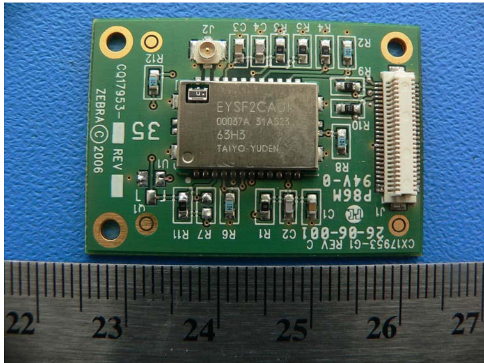
EUT – Transceiver component side view
