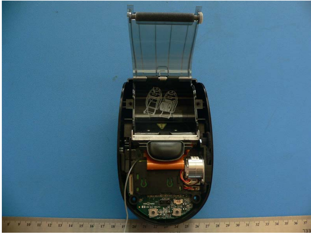
EUT – Chassis off view
