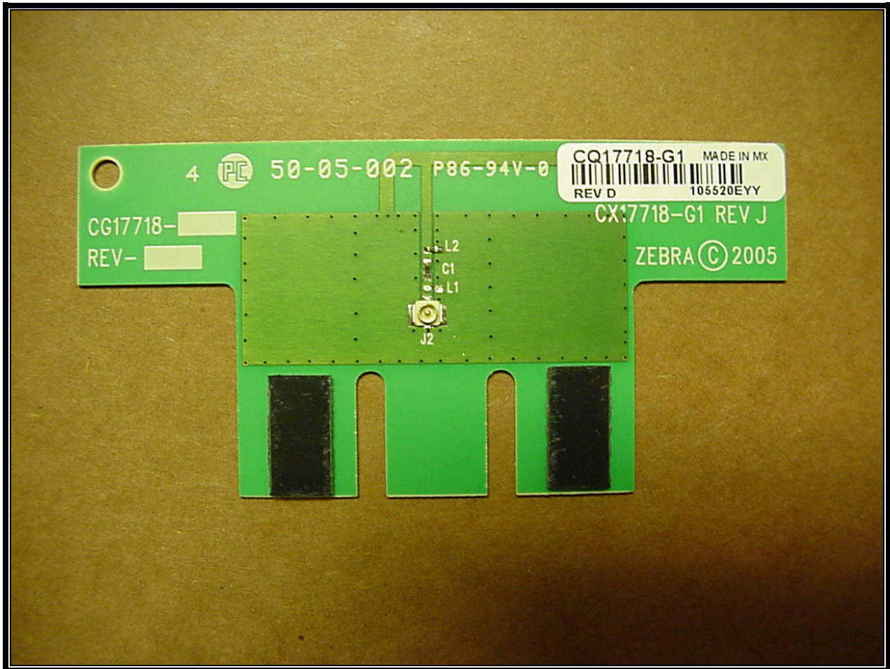
Photograph 11: CQ17718-G1 Antenna – Top View
