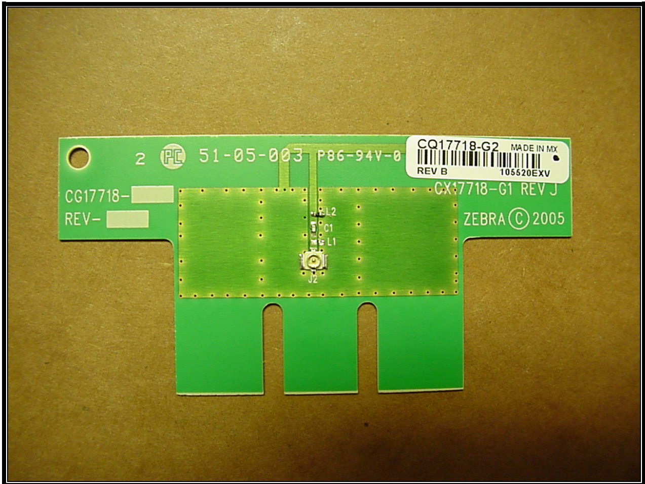
Photograph 13: CQ17718-G2 Antenna – Top View
