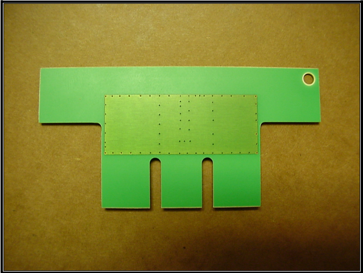
Photograph 14: CQ17718-G2 Antenna – Back View
