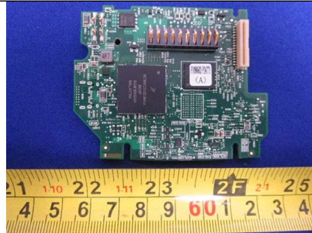
PCBA A – Bottom View
