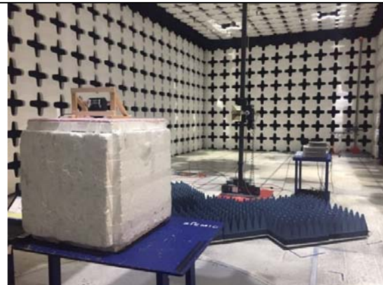
Radiated Emissions (>1GHz) – Rear View (EUT vertical)
