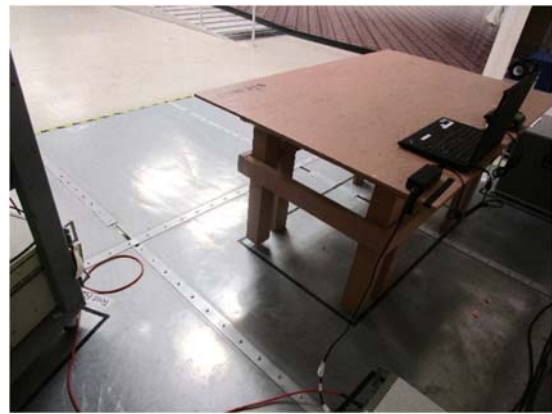
AC Line Conducted Emissions – Rear View
