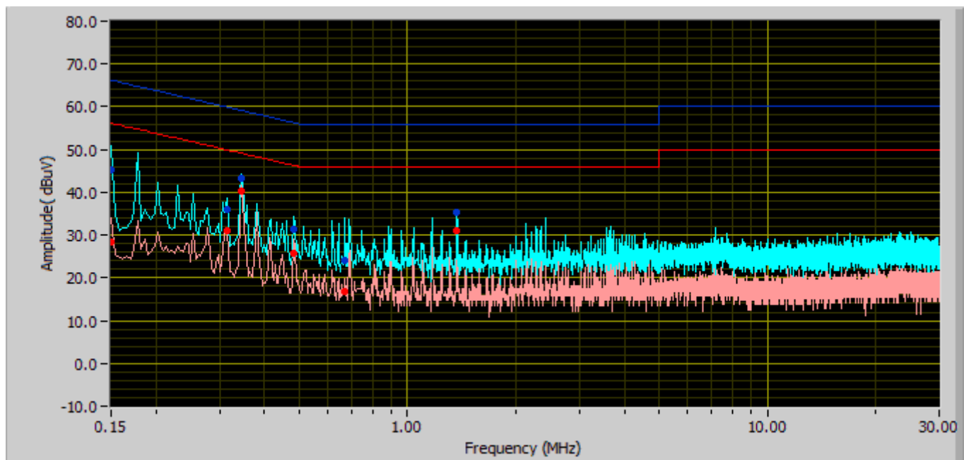
Neutral Line Plot at 120Vac, 60Hz
