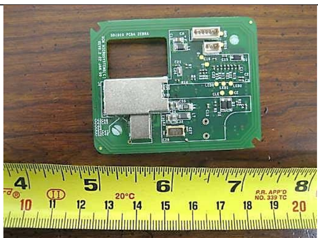
PCBA6 with Shielding Bottom View
