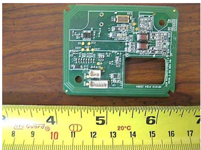
PCBA6 without Shielding Bottom View 1
