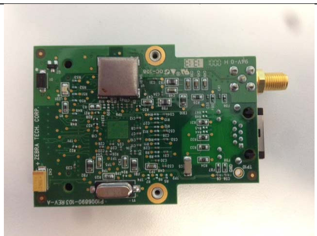
WLAN Radio Board Bottom View
