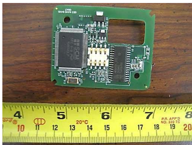
PCBA6 without Shielding Top View
