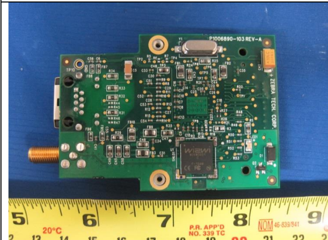
EUT – Shielding off View
