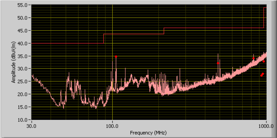
Radiated Emission Plot (Receive mode)
