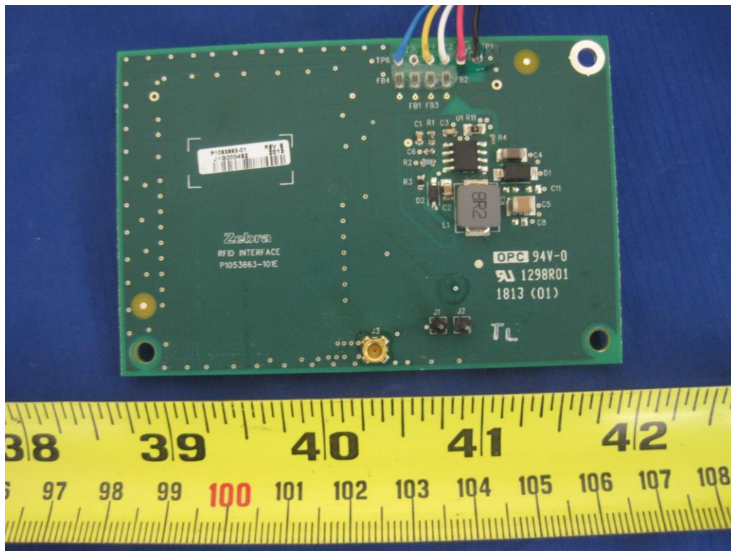
RFID Module-Top View
