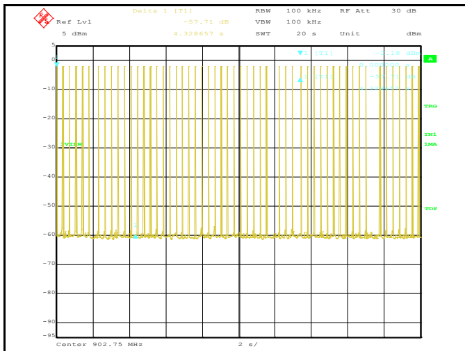
Low Channel (Sweep in 20sec)
