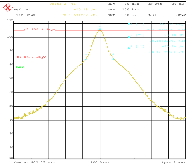
20dB Occupied Bandwidth -Low Channel
