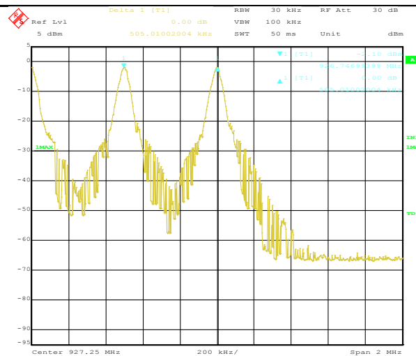
Channel Separation-High Channel
