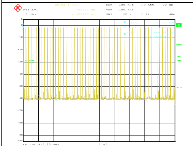
Middle Channel (Sweep in 20sec)
