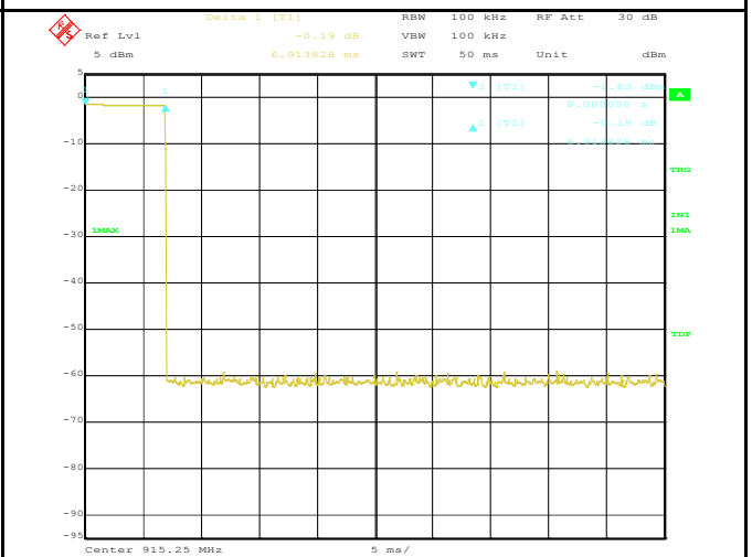
Mid Channel (Sweep in 50msec)
