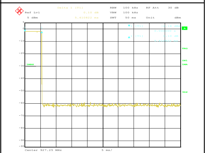
High Channel (Sweep in 50msec)
