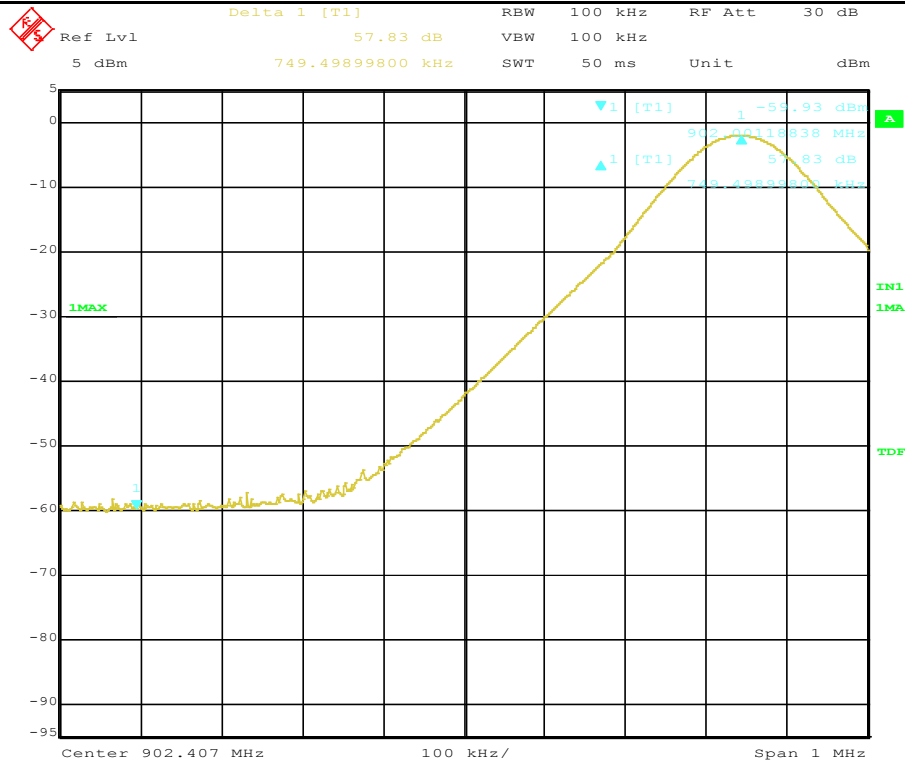
100 KHz Bandwidth of Frequency Band Edge-Low Channel
