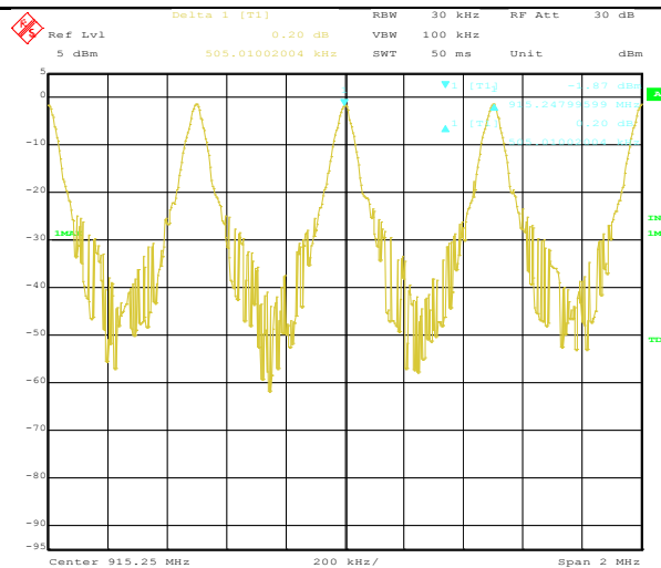
Channel Separation-Mid Channel
