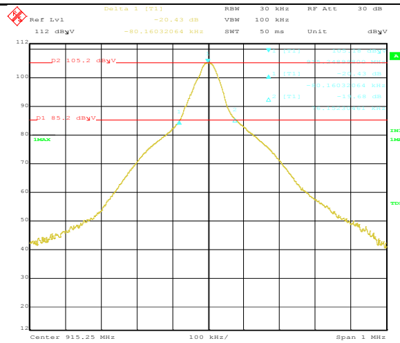
20dB Occupied Bandwidth -Mid Channel
