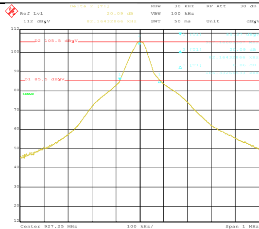
20dB Occupied Bandwidth -High Channel
