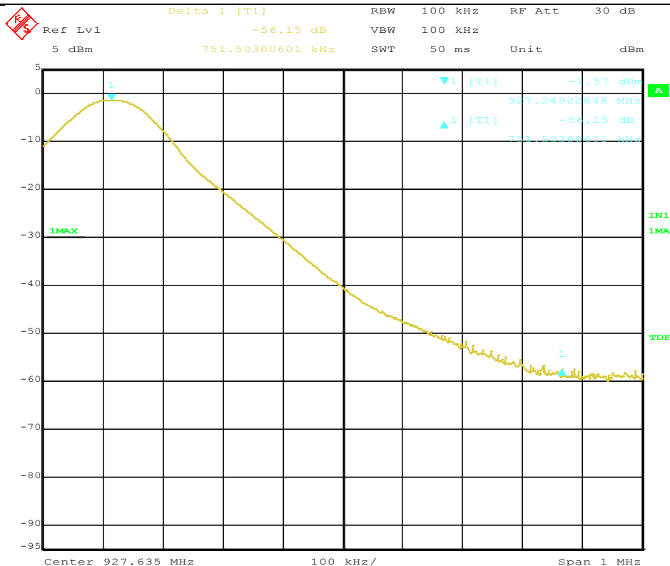
100 KHz Bandwidth of Frequency Band Edge -High Channel
