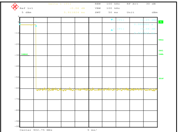
Low Channel (Sweep in 50msec)
