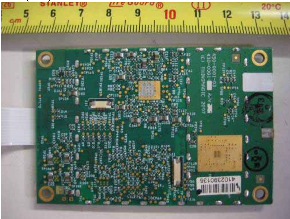
RFID (UHF) Module Solder View
