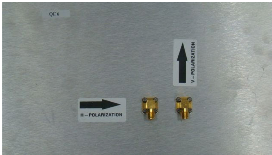
Panel Antenna : MA-WA56-DPIP – Bottom view with connectors
