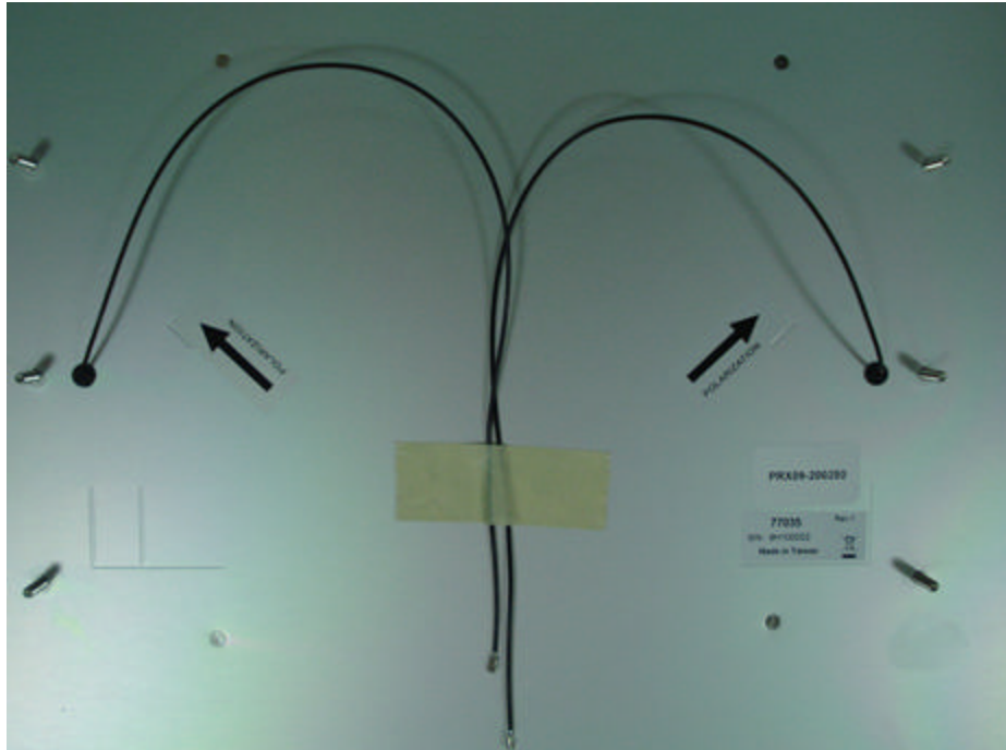
Panel Antenna : PRX09-200250 – Bottom view
