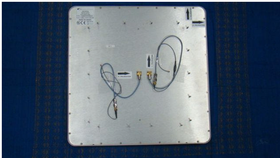
Panel Antenna : MA-WA56-DPIP – Bottom view
