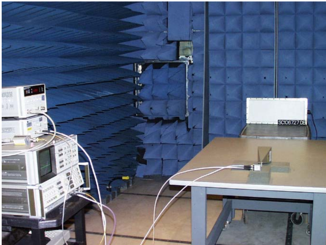
Photograph of Test Setup: Radiated Emissions in Restricted Bands
