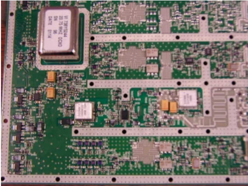
RF board, oscillator detail (above).
