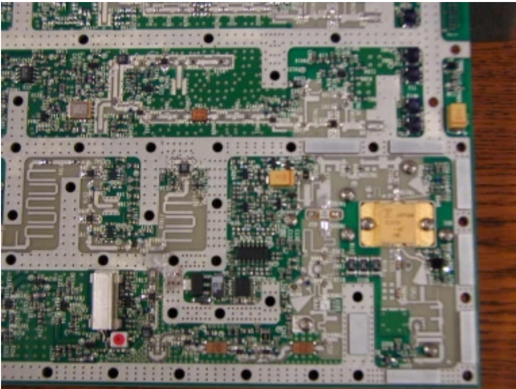
RF board, power amplifier detail (above).
