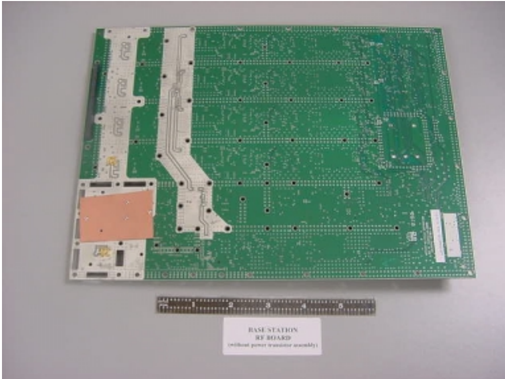
RF board, solder side (above).
