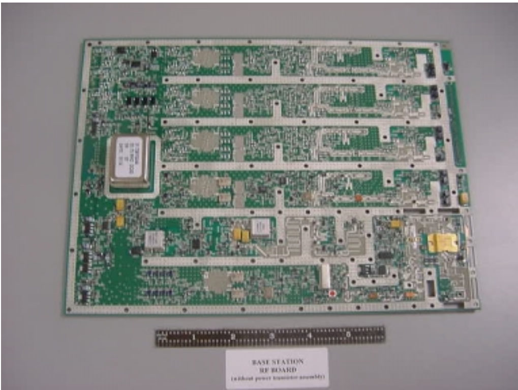
RF board, component side (above).
