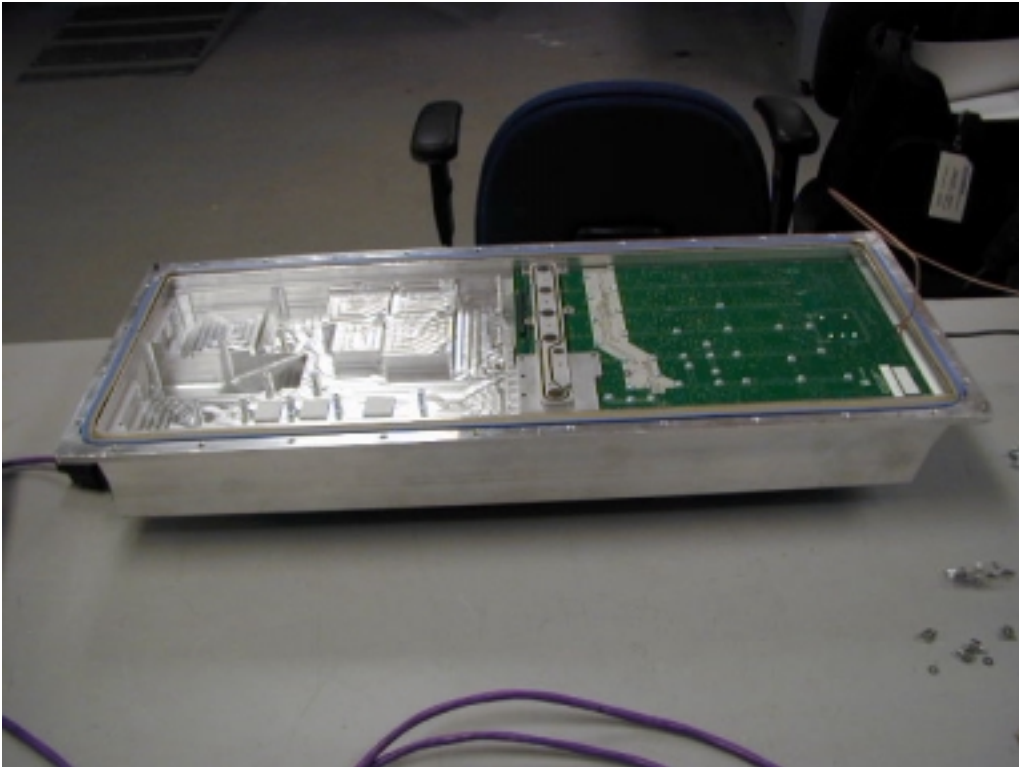
Base, partially populated (above).
