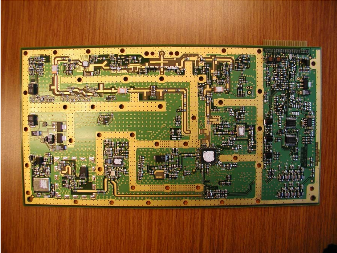
RF Board Side 1
