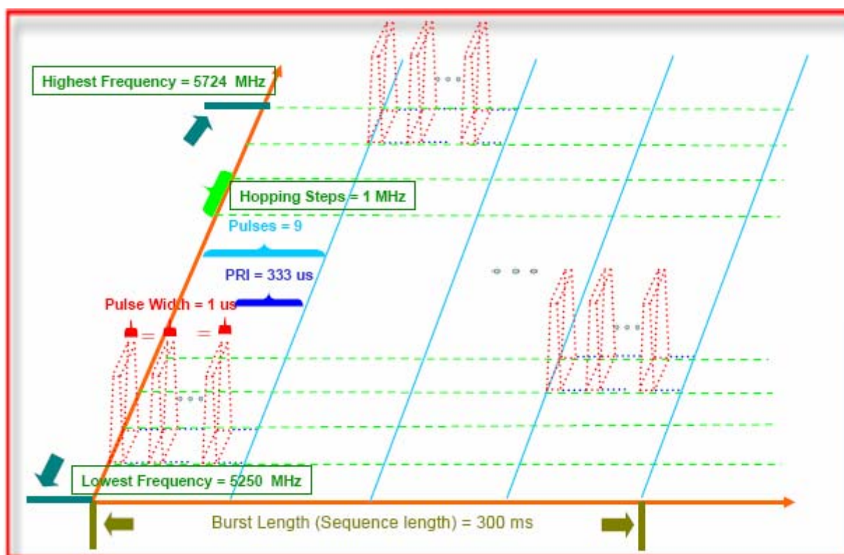
FCC Radar Types (6) System Diagram
