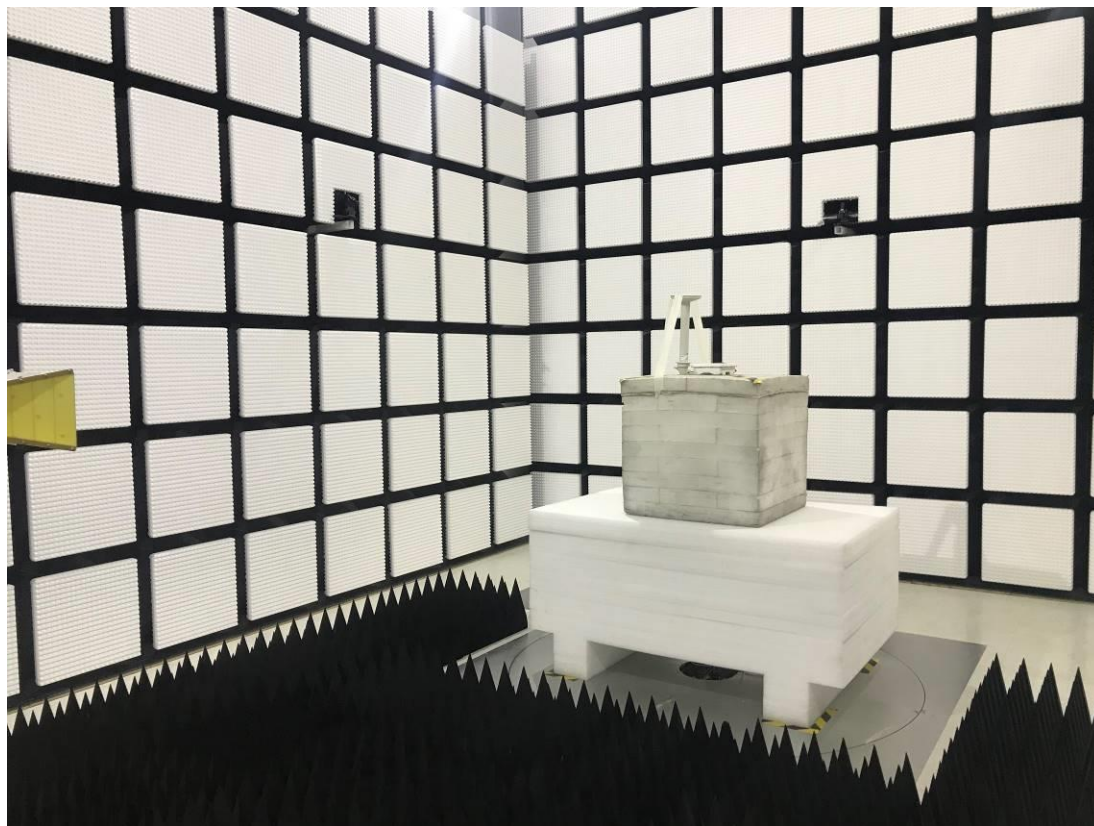
Radiated Emission Above 1GHz View -34dBi
