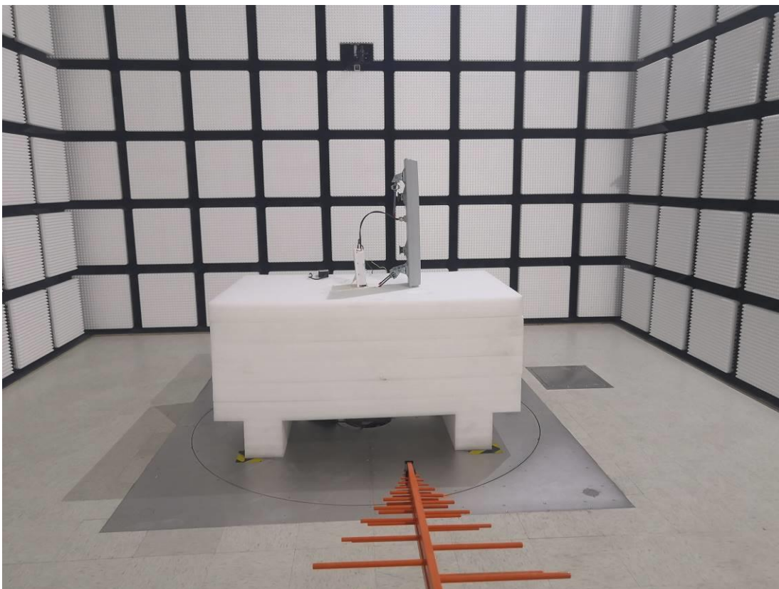
Radiated Emission Below 1GHz View - 21dBi
