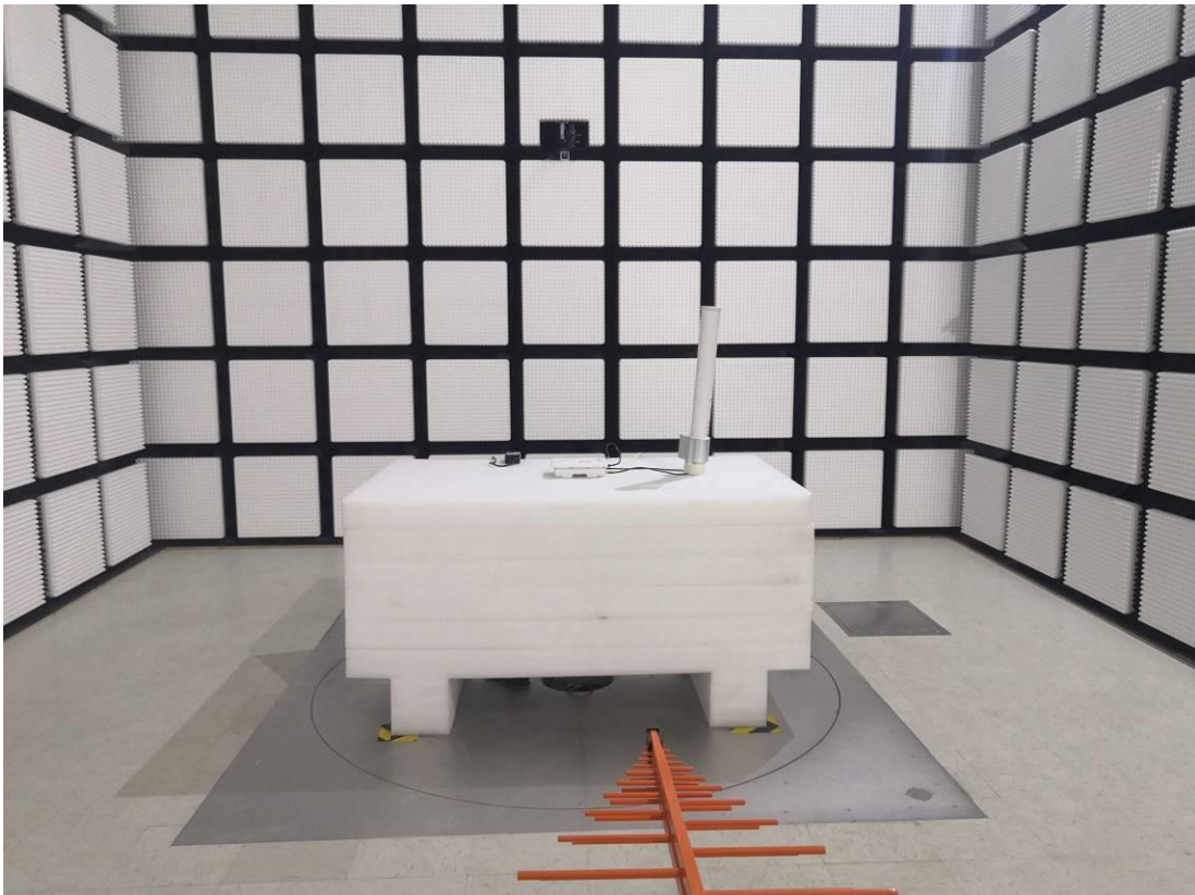
Radiated Emission Below 1GHz View - 13dBi
