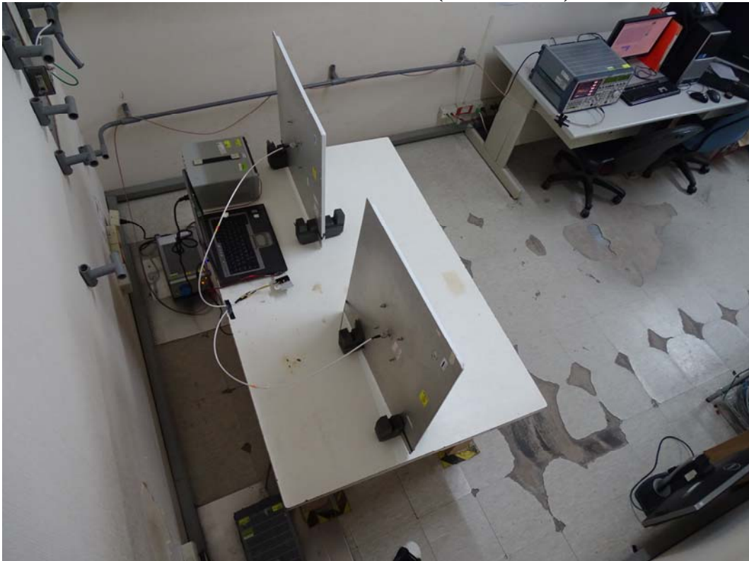
Back View of Conducted Test (Panel Antenna)
