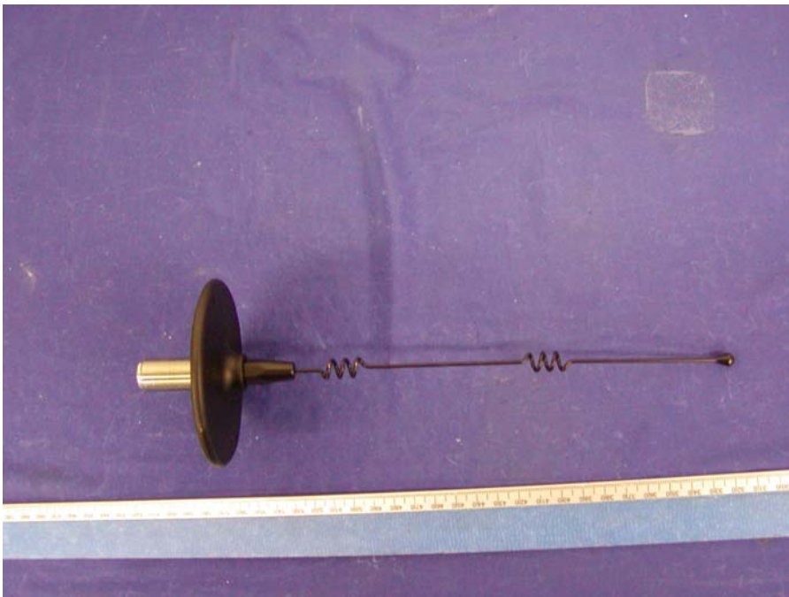
Antenna 2449LT Side View
