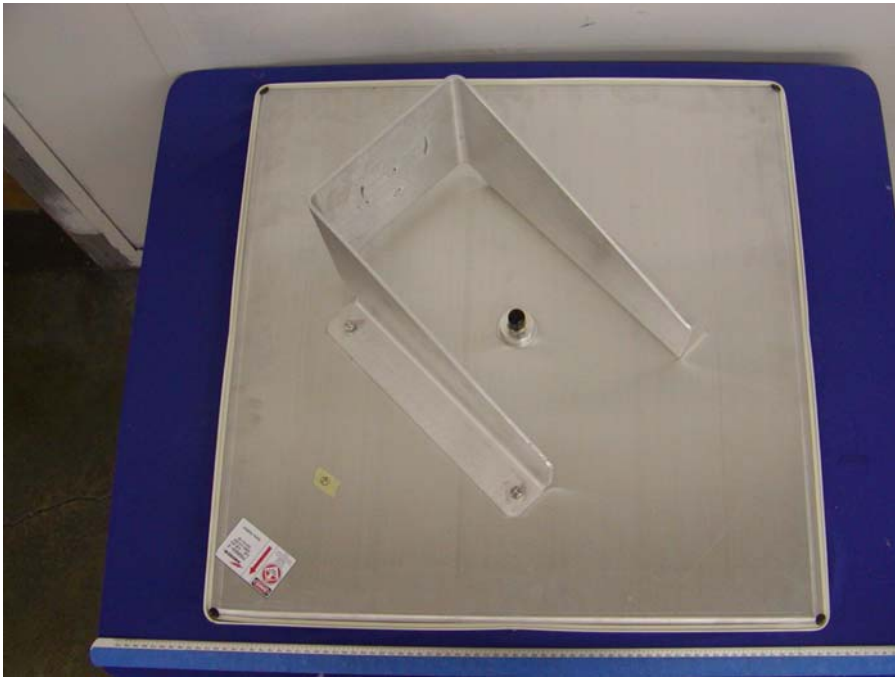
Antenna R0320-100
