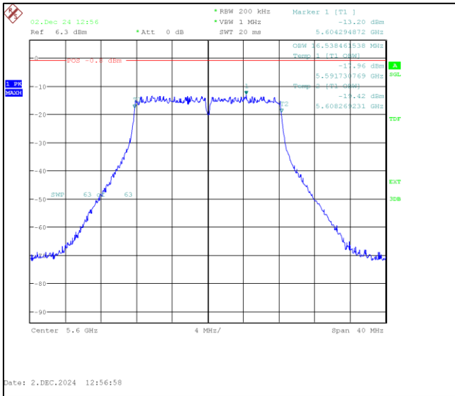
Channel Frequency:5600MHz
