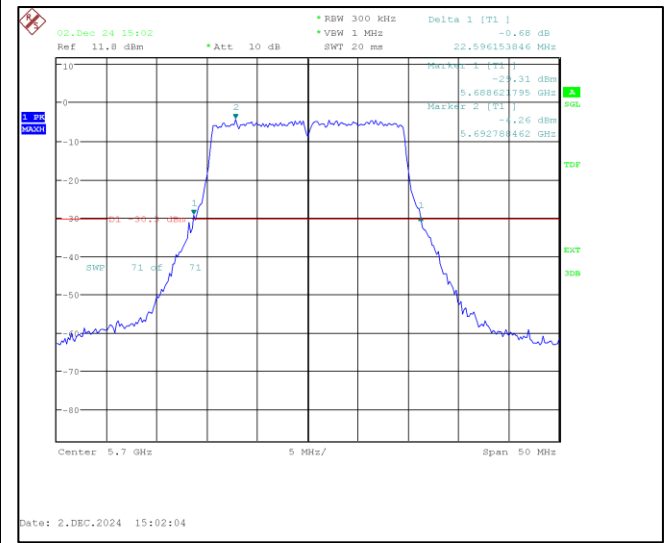
Channel Frequency:5700MHz
