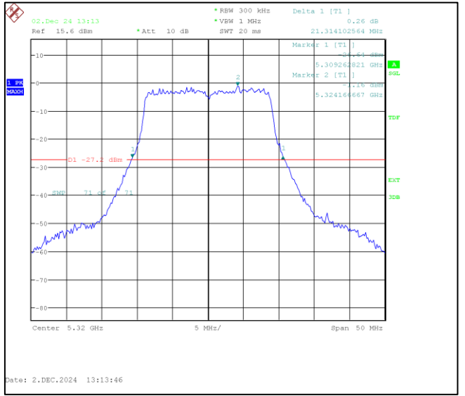
Channel Frequency:5320MHz
