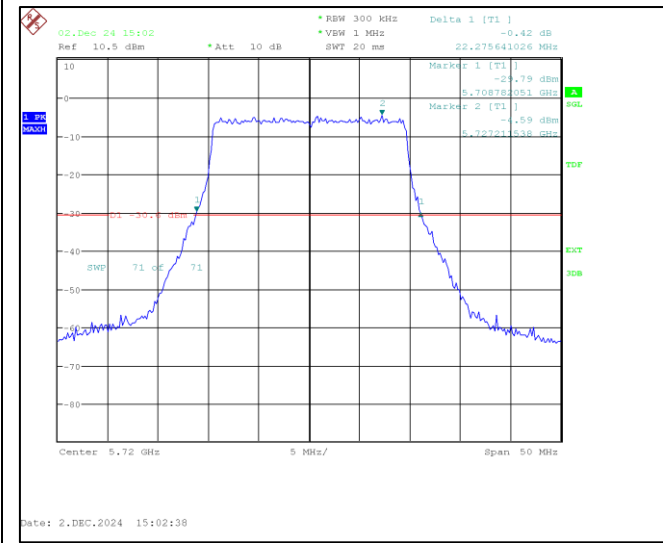
Channel Frequency:5720MHz
