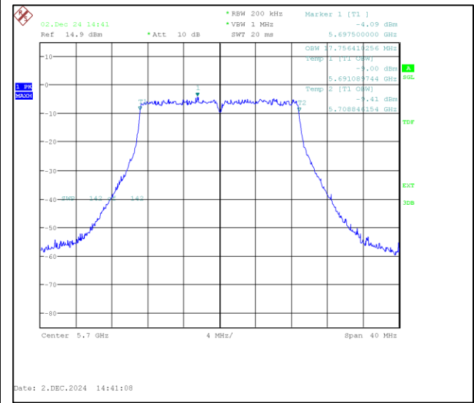
Channel Frequency:5700MHz
