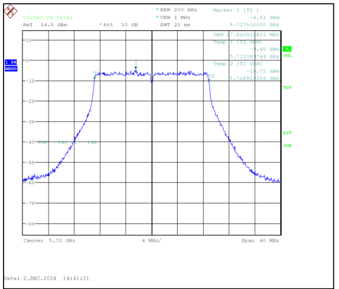
Channel Frequency:5720MHz
