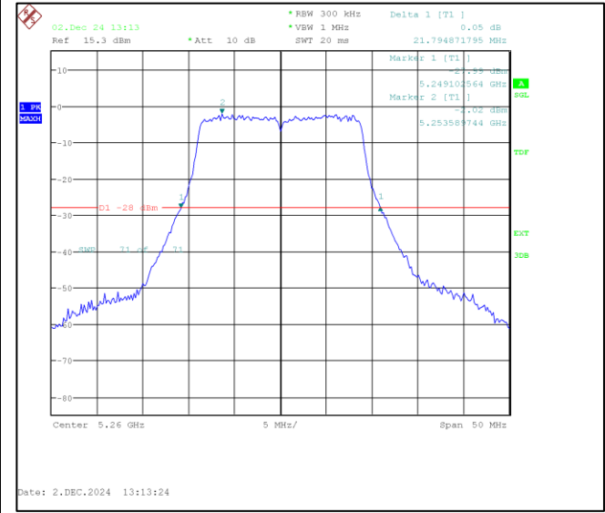
Channel Frequency:5260MHz
