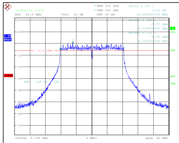
Channel Frequency:5745MHz
