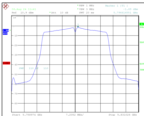
Channel Frequency:5795MHz
