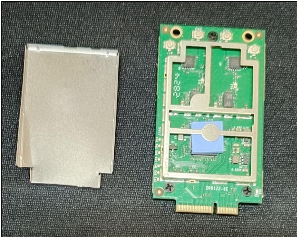
Module with encloser
