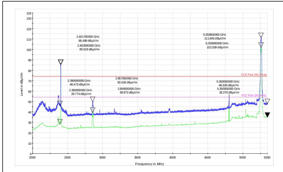
Vertical Polarization
