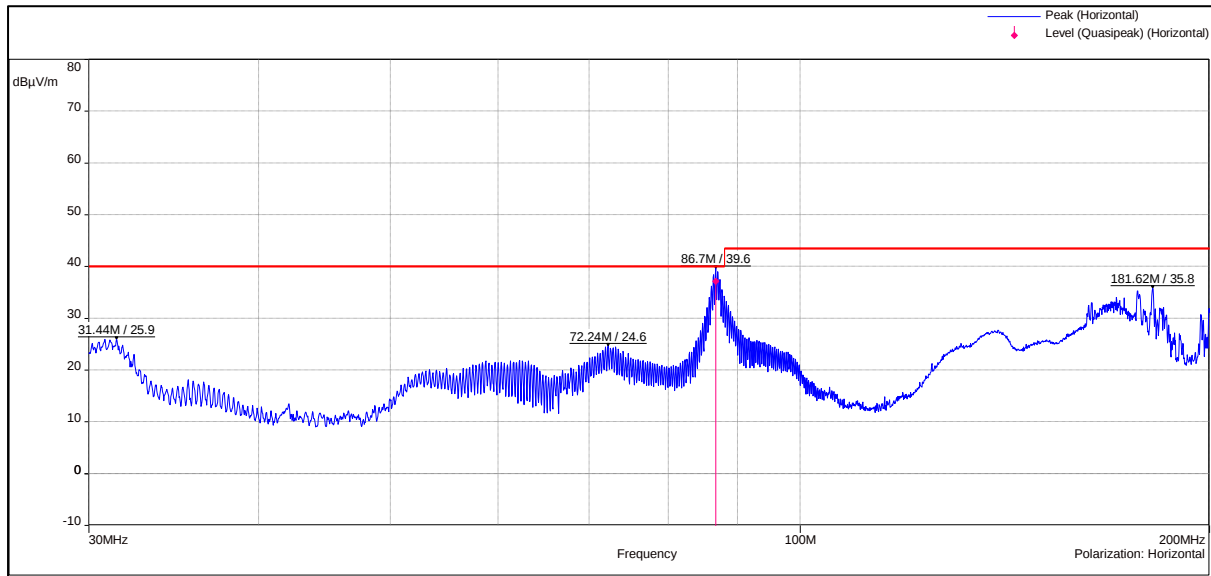
Channel Frequency 30MHz – 200MHz
