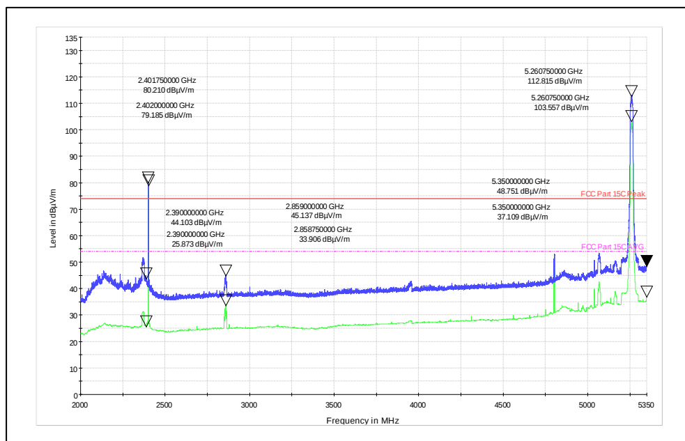
Horizontal Polarization
