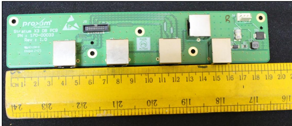
Daughter Board Dimensional View
