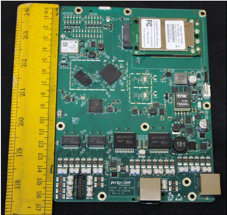
SX3 PCB Dimensional View
