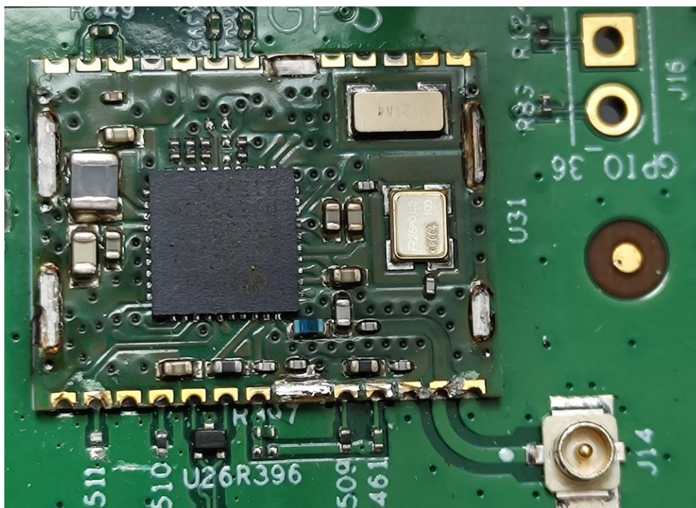
GPS Module Close-Up View without Shield
