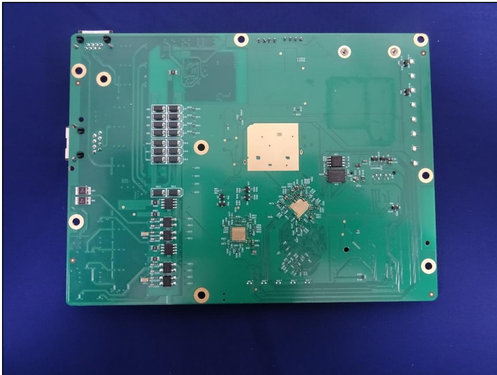
SX1 PCB Rear View
