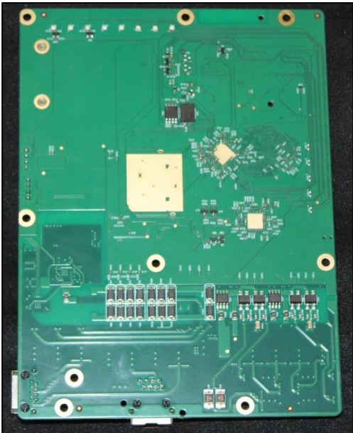
SX3 PCB Rear View
