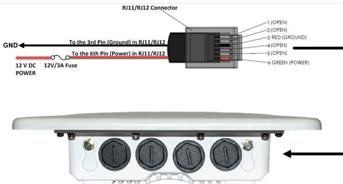
Figure 3-3 Powering the device through Access Port using 12 V DC Power Supply
