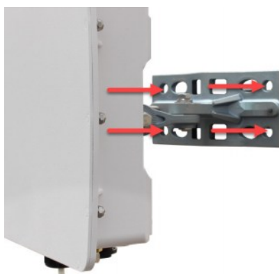
Figure 4-4 Pole Mounting
