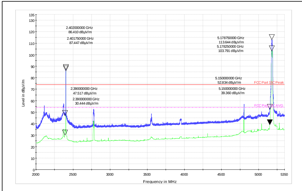
Vertical Polarization
