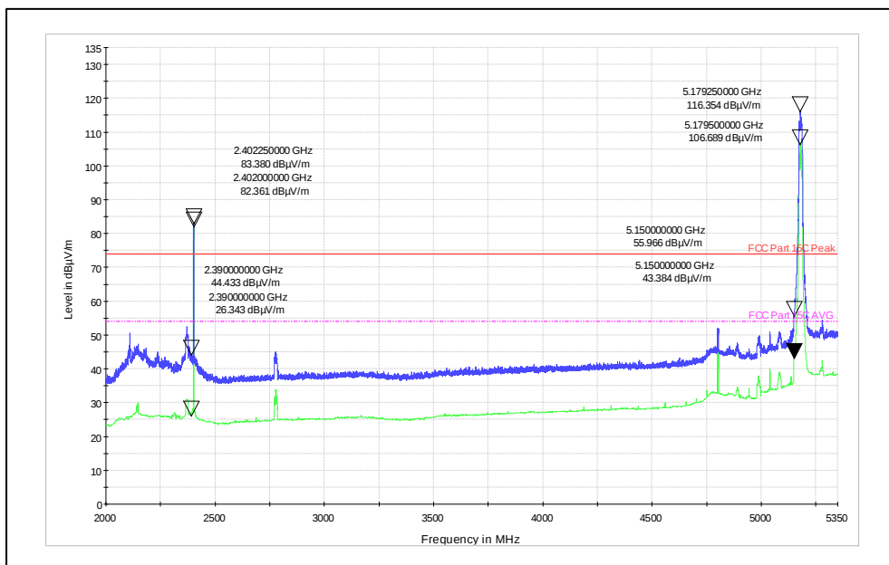
Horizontal Polarization
