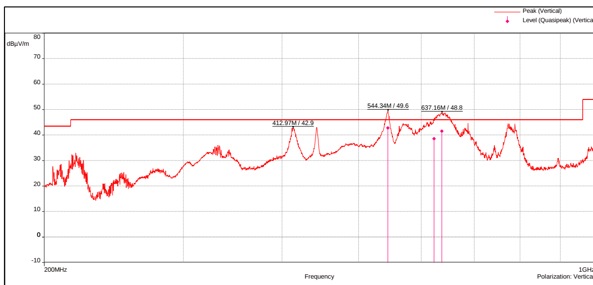
Channel Frequency 200MHz – 1GHz
