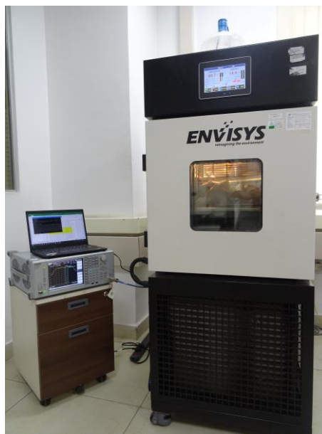
Temperature@+60°deg
