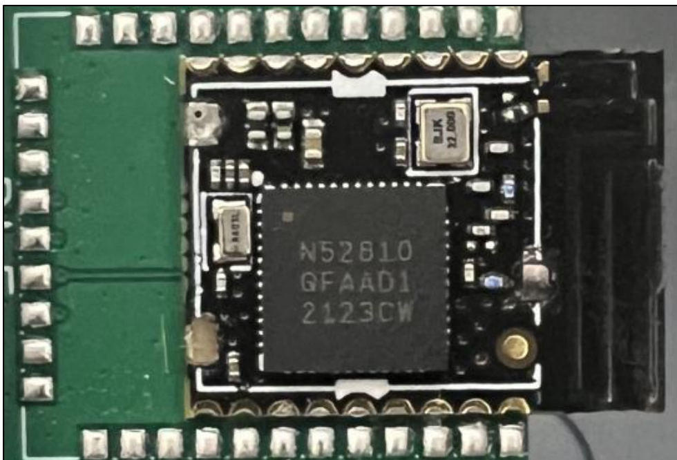
BLE Module without Shield close up View
