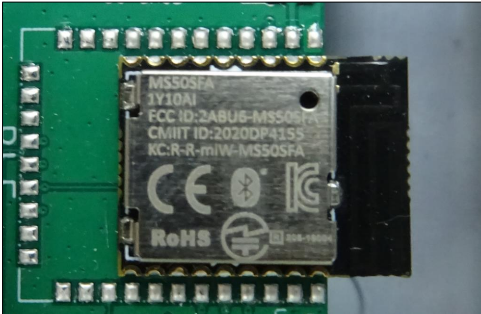
BLE Module with Shield Close up View
