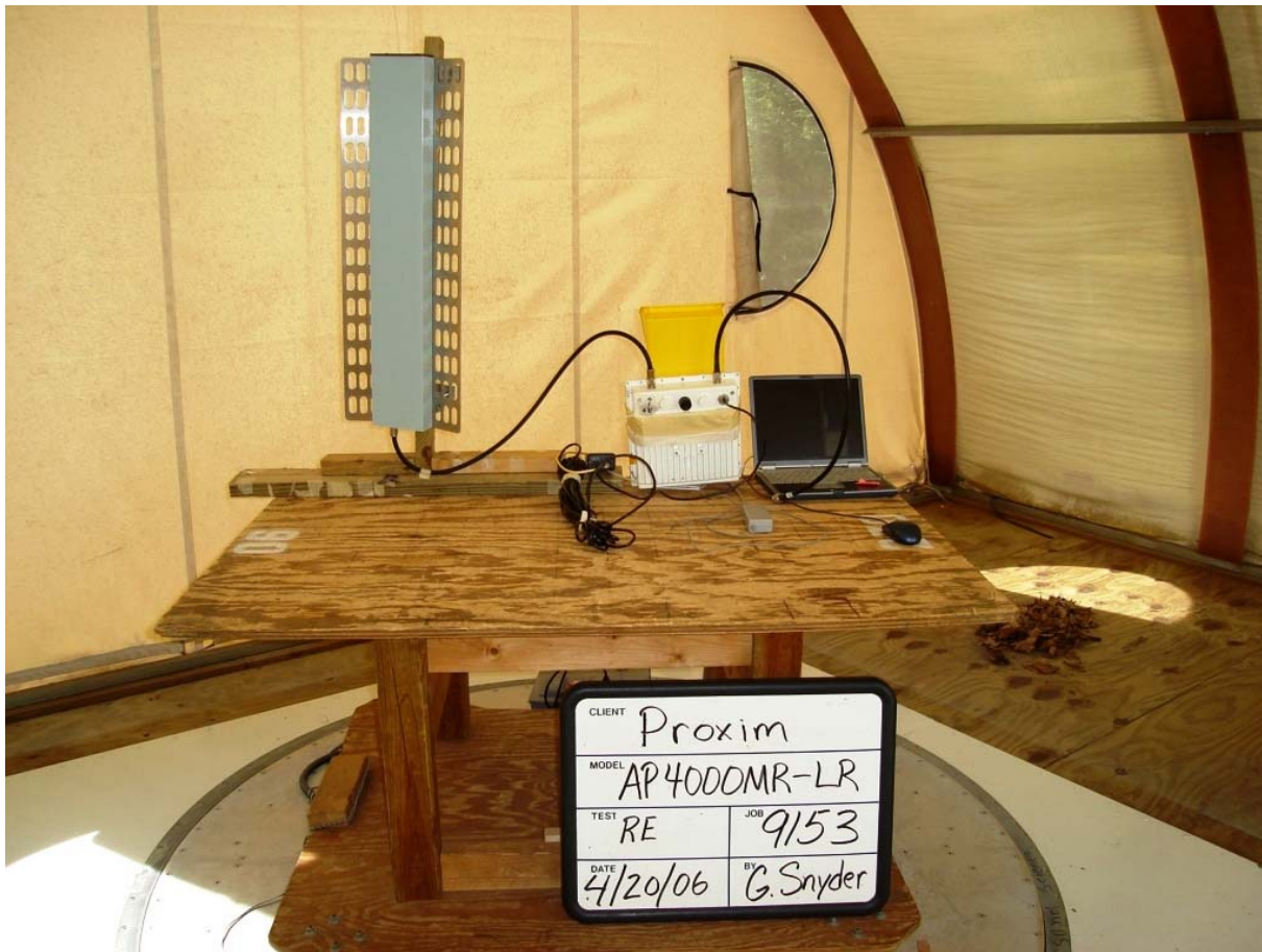
Figure 2. A245LP17 Antenna
