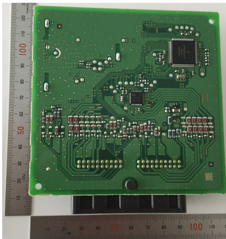
Antenna side
