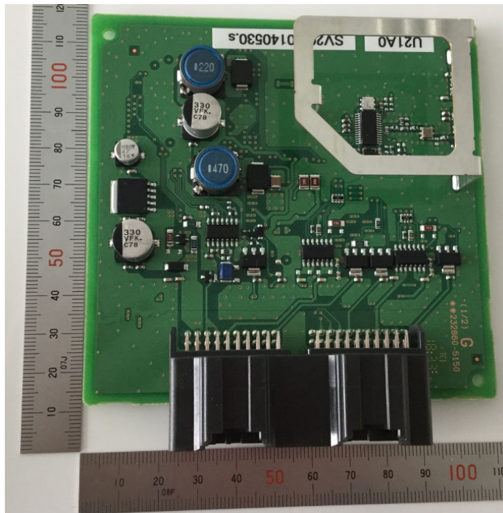
Component side
