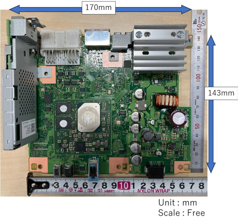
Component Side(Cockpit Control Unit) – Main PCB
