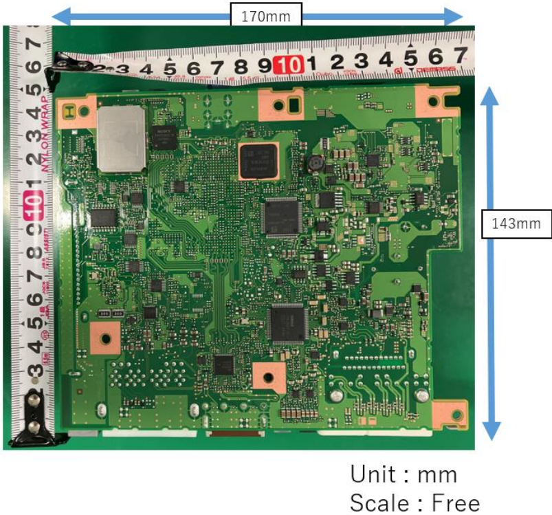
Solder Side(Cockpit Control Unit) – Main PCB
