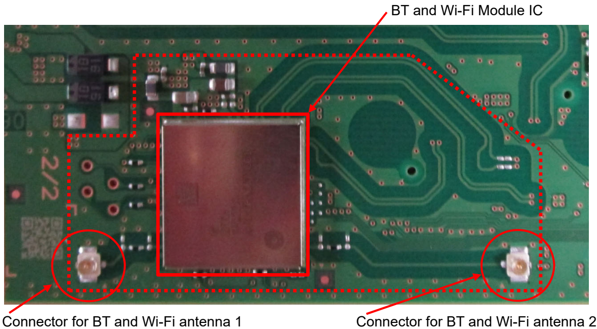
BT and Wi-Fi Module IC (Top view without cover)
