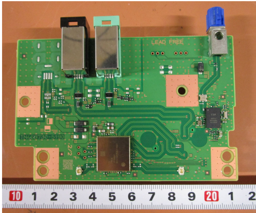
Component Side
