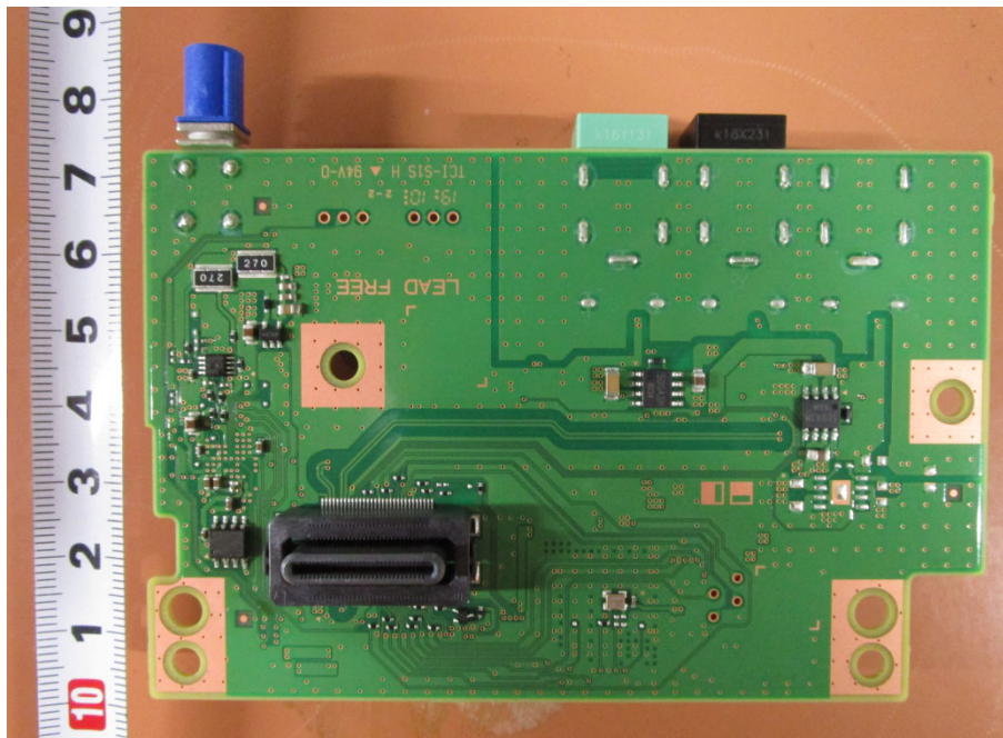
Solder Side
