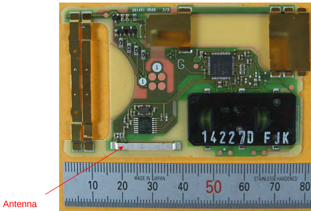
Component Side
