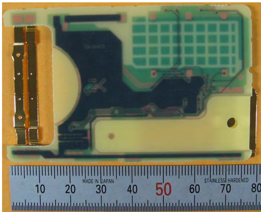
Solder Side
