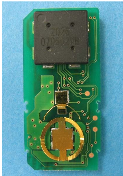
Solder Side
