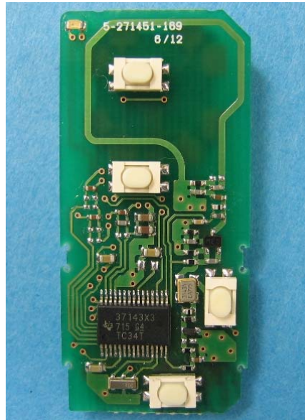
Comp Side
