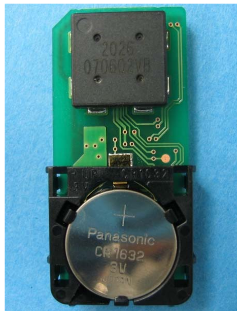
Sold Side
