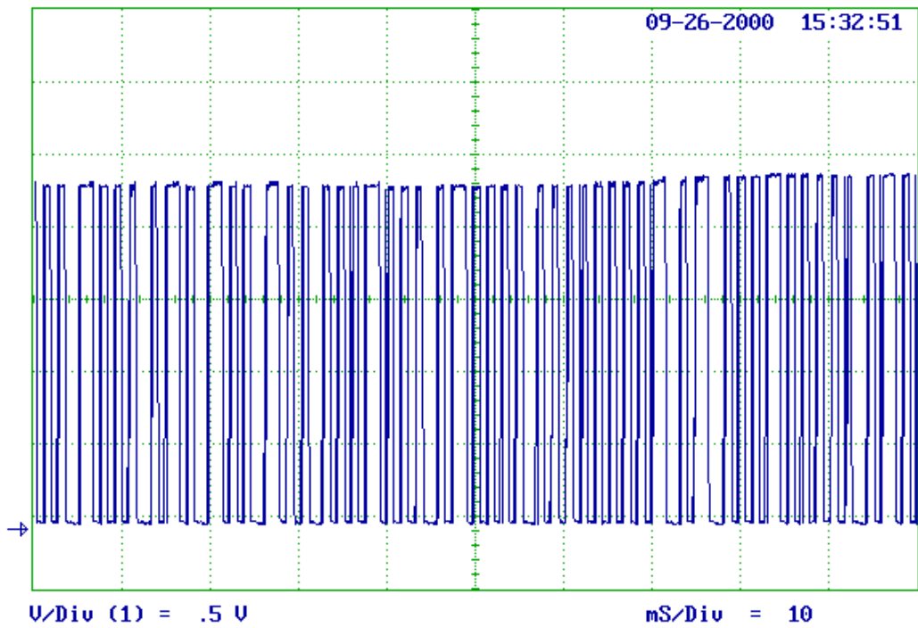
DUTY CYCLE FOR 12BAN - 10 WIDE PULSES + 42 NARROW PULSES
