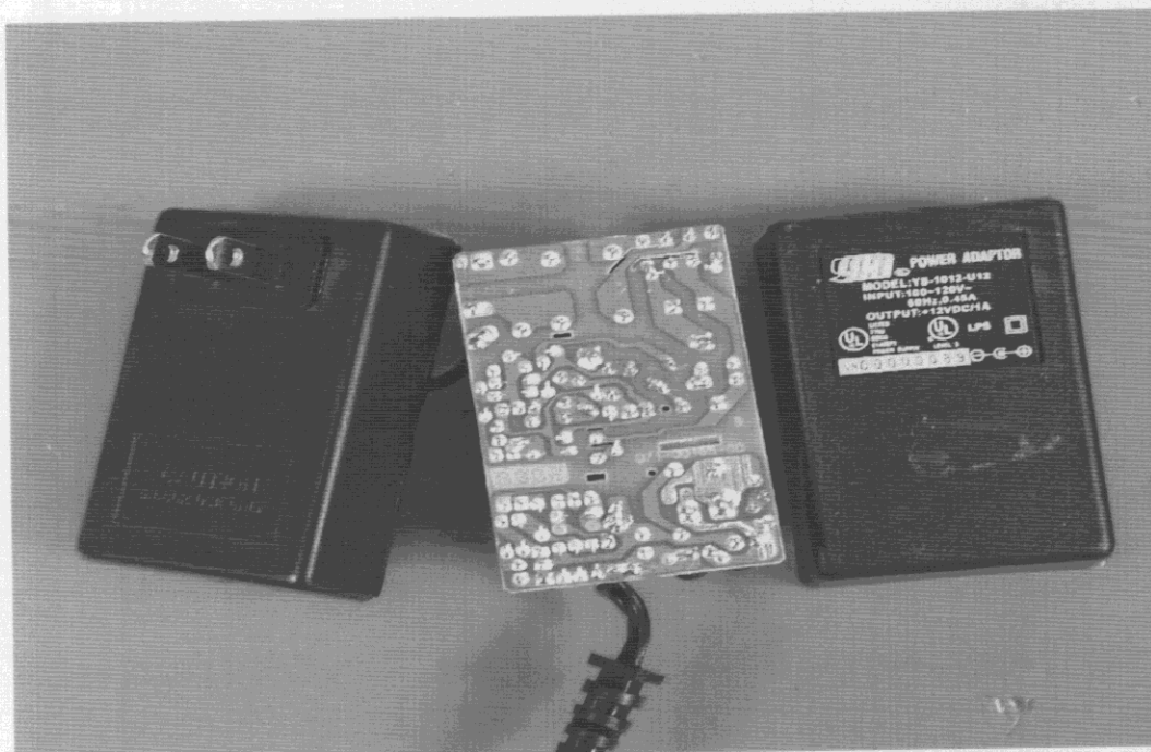
Mode 2:Back View of Adaptor
