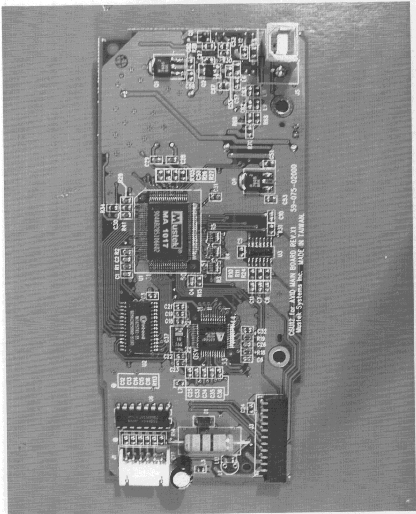
Component Side View of Main Board
