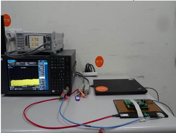
Part_15_209_EMR_Radiated_Setup
