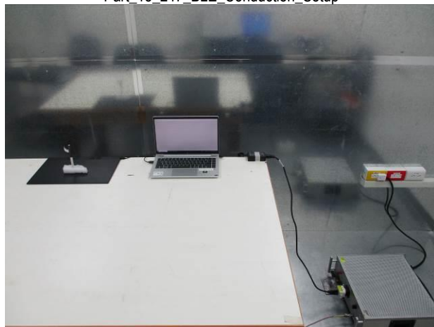
Part_15_247_BLE_Conduction_Setup
