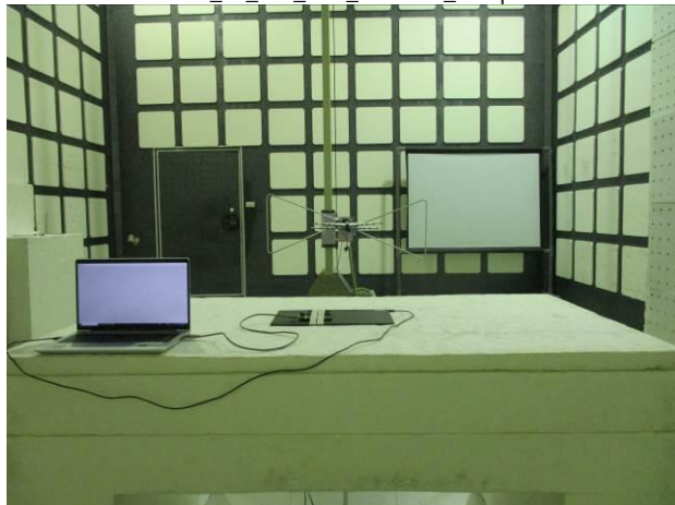
Part_15_247_BLE_Radiated_Setup
