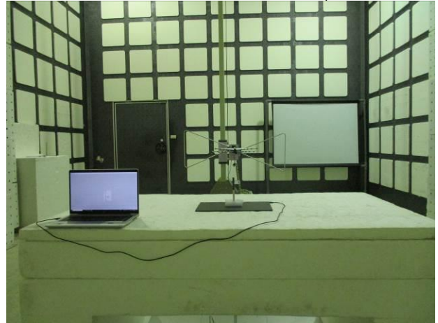
Part_15_209_EMR_Radiated_Setup
