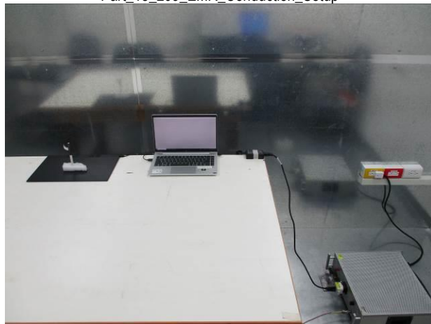
Part_15_209_EMR_Conduction_Setup
