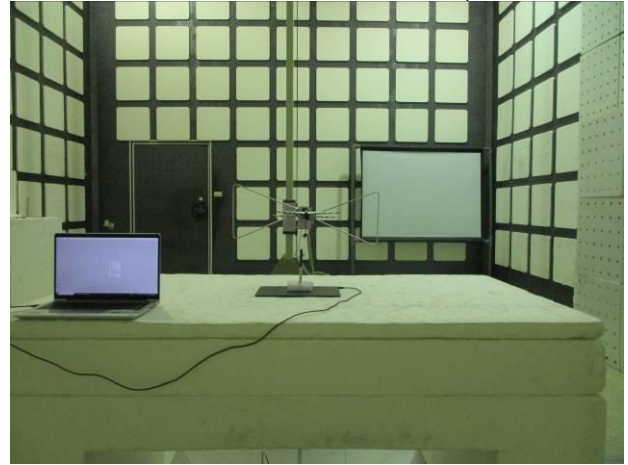
Part_15_211_EMR_Radiated_Setup
