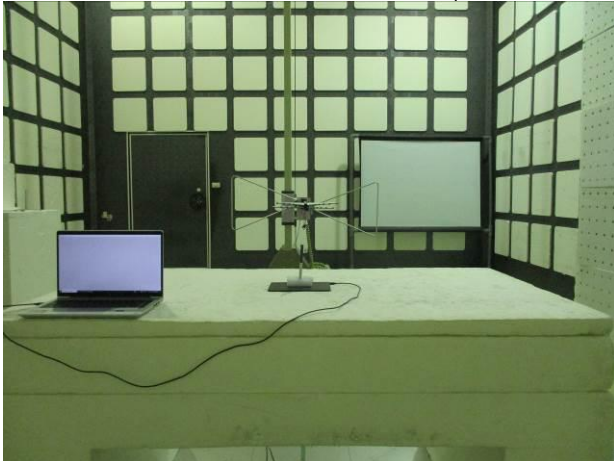
Part 15.209_EMR_Radiated_Setup
