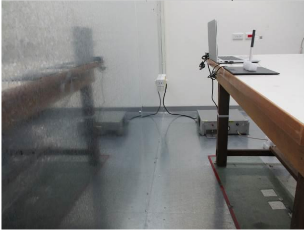
Part_15_247_BLE_Conduction_Setup
