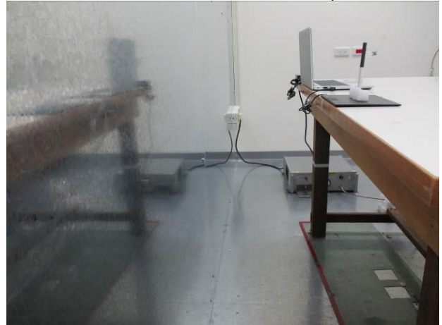
Part 15.209_EMR_Conduction_Setup
